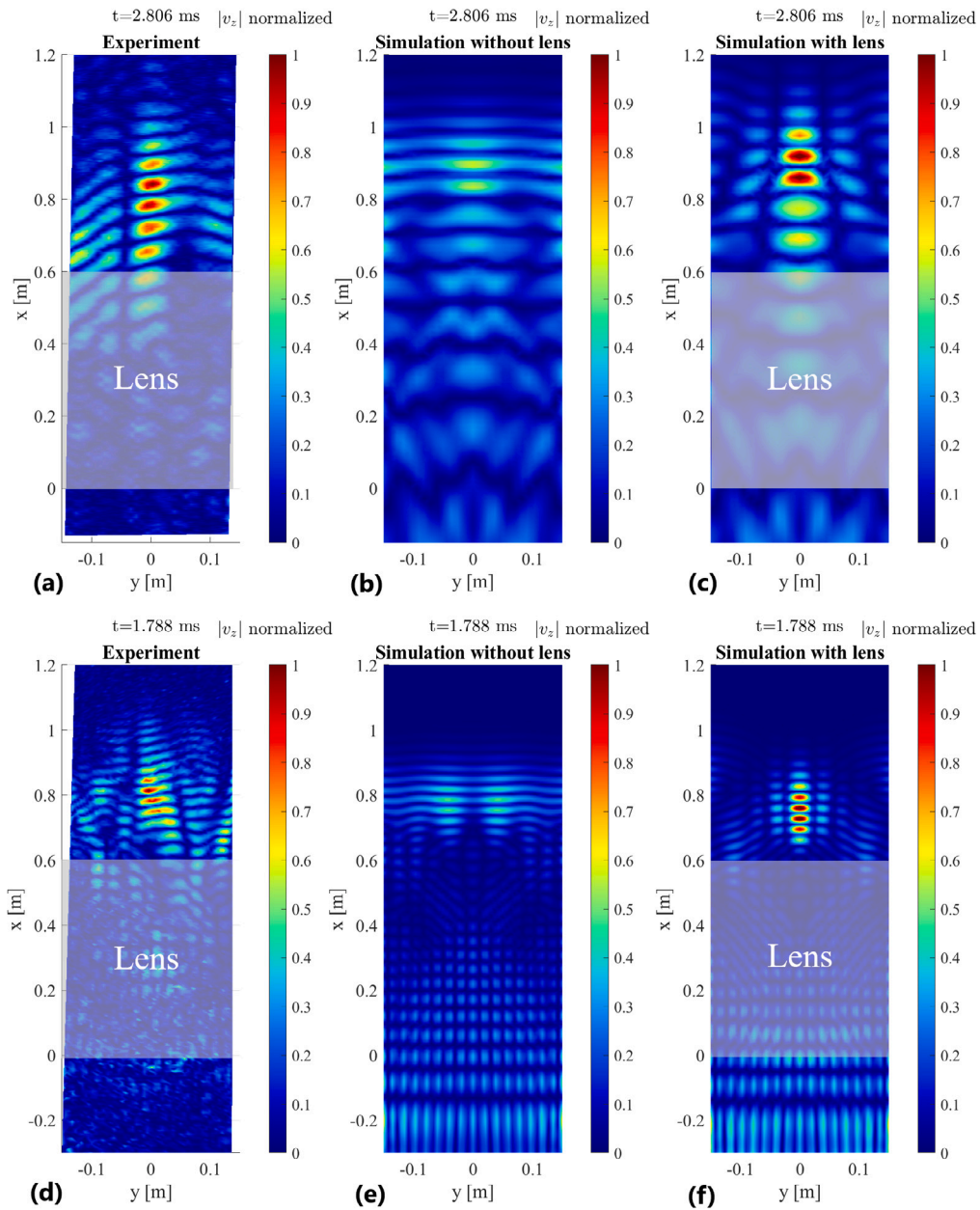
Fig. 14. Comparison of normalized absolute out-of-plane wave field velocity for an incident plane flexural wave at focusing time for two frequencies: 2000 Hz. For 2000 Hz, (a) experimental result of the manufactured plate with a composite lens structure, measured using a scanning laser Doppler vibrometer ( Polytec PSV-500-H ); (b) shows numerical result of a plate without lens and (c) shows numerical result of a plate with lens. For 8000 Hz, (d), (e), and (f) present the same comparisons, respectively; See supplementary data for the wave propagation video .
