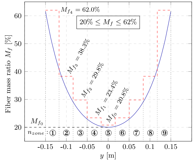
Fig. 2. Fiber mass ratio gradient for a UD carbon-epoxy composite plate, according to Eq. (6) with M_{f_0} = 20\% , f_l = 0.3 m and n_0 = 1 (blue continuous line) and discretized gradient in n = 9 sectors (red dashed line).
