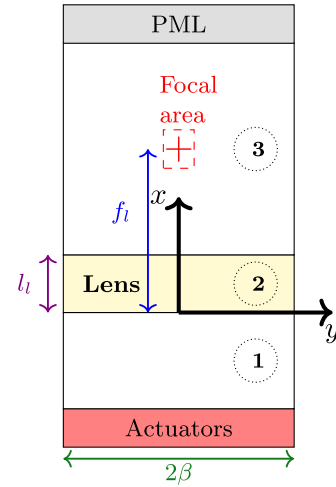
Fig. 1. Top view of GRIN-Lens (zone ②: material properties y gradient) in a host plate (zones ① and ③).
