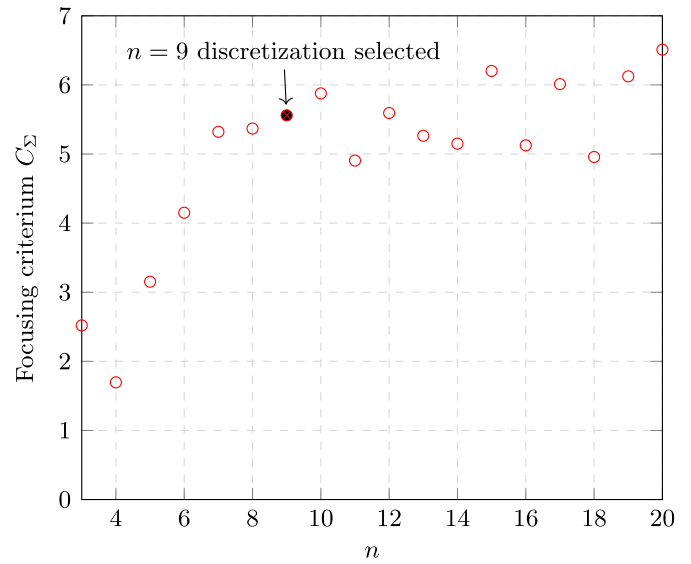
Fig. 7. Effect of gradient discretization on the focusing performance for f = 8000 Hz; Performance criterion C_e described in Section 4.2.
