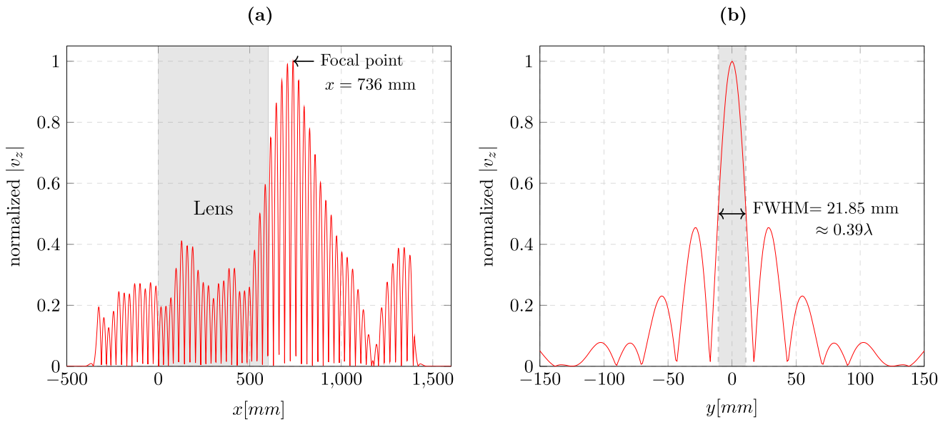
Fig. 11. (a) Normalized absolute out-of-plane velocity |v_z| along x -axis for f = 8000 Hz; (b) Full Width at Half Maximum criterion for f = 8000 Hz at x = 736 mm.
