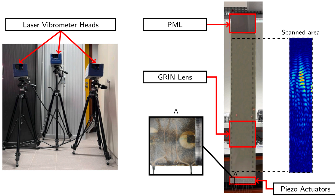
Fig. 12. Experimental setup.
