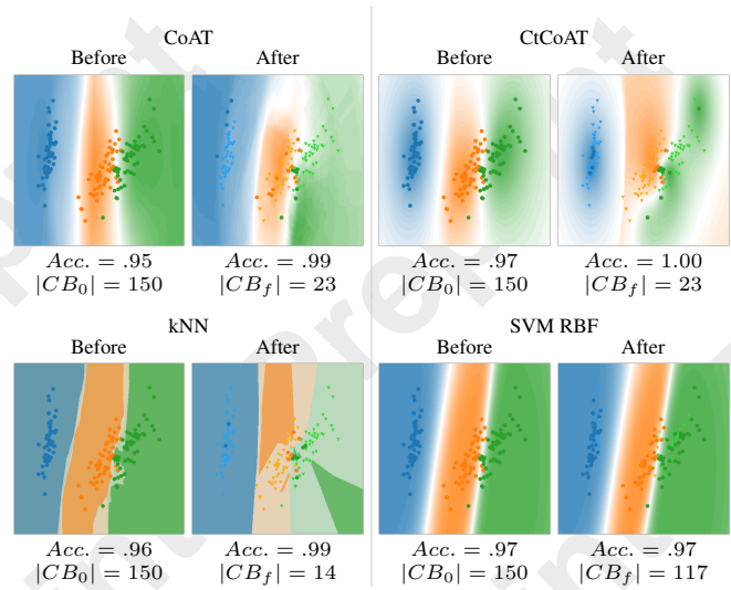
Figure 1: Sculpting the decision frontier by removing cases using EnergyCompress: improving both accuracy and inference time through case base compression (Iris dataset, 2D PCA projection).
