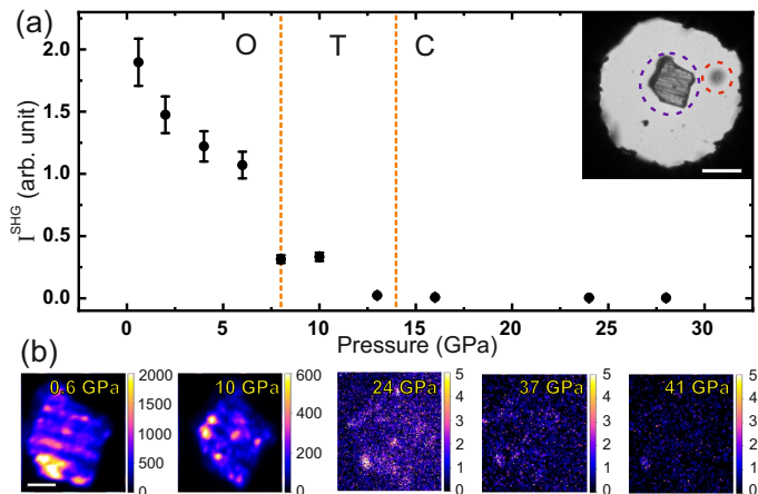
Figure 3. Variation of the second-harmonic generation (SHG) response with pressure. (a) Overall isotropic intensity variation. Dashed lines separate pressure ranges corresponding to the different phases. The inset displays an optical microscopy image showing the sample (blue dashed circle) and the ruby ball (red dashed circle). (b) SHG microscopy images of the sample at selected pressures. The scale bar is 10 \mu\text{m} .
