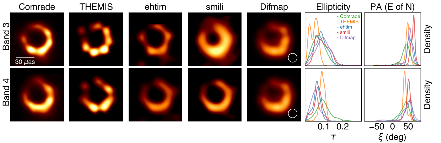
Fig. 5. EHT 2018 M87* images and ellipticity ( \tau ) and ellipticity position angle ( \xi ) distributions. (left to right) Images from each imaging method (Comrade, THEMIS, eht-imaging, SMILI, and DIFMAP). For Comrade and THEMIS, mean posterior images are shown. Fiducial images from the respective Top Sets are shown for the other methods. The two right panels show the distributions of \tau and \xi for each method. Top and bottom rows show results for band 3 and band 4, respectively. Colors correspond to each method (see legend).
