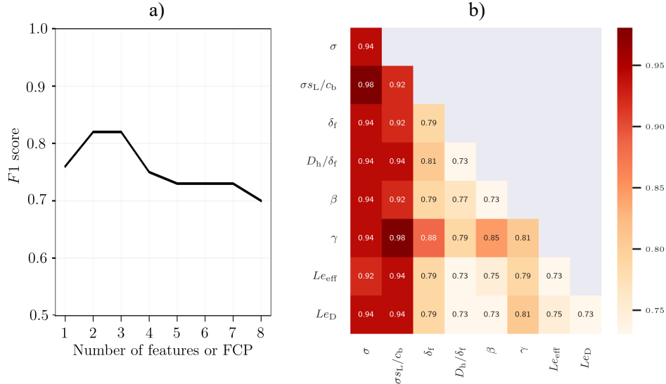
Figure 2: Recursive Feature Elimination results with Logistic Regression (a) Average F1 score, and (b) auto- F1 score matrix, where each number represent the test accuracy for the respective pair of FCP. The main diagonal corresponds to the F1 score using a single FCP only.
