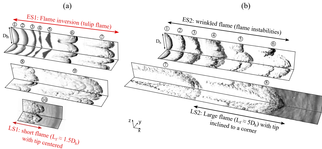
Figure 1: Characteristic flame morphology during flame acceleration (FA), (a) ES1 → LS1, and (b) ES2 → LS2 transition.
