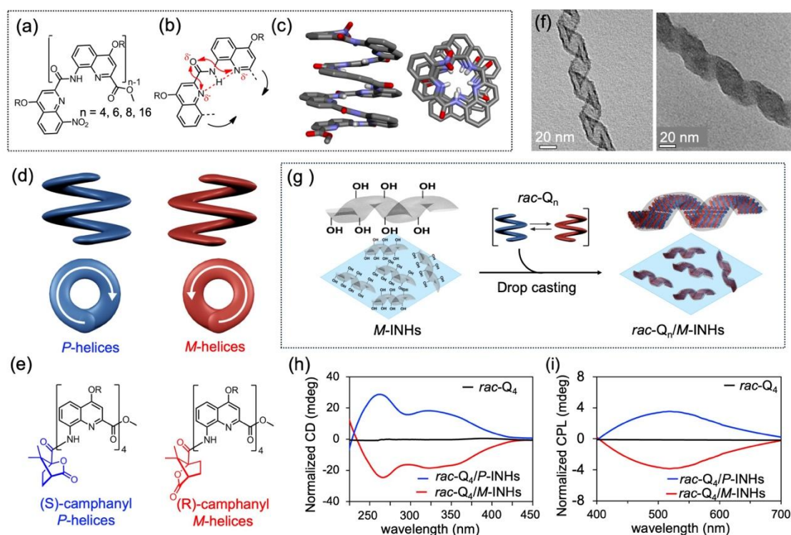
Fig. 1 (a) Chemical structure of a rac-Q_n ( n = 4, 6, 8, 16 ) sequence with a nitro group at the N-terminus. (b) Folding principle of rac-Q_n oligomers; hydrogen bonds (---) are shown in red dotted lines whereas electrostatic repulsions ( \leftrightarrow ) are indicated with red arrows. (c) Side- and top-view of the X-ray structure of Q_8 . Sidechains, hydrogens and solvent molecules are removed for clarity. 34, 35 (d) Schematic representation of a P - and a M -handed helices. (e) Formula of P - Q_4 (blue) and M - Q_4 (red). (f) TEM image of INHs before (left) and after (right) drop-casting rac-Q_4 . (g) Illustration of the drop-casting approach of racemic oligoamide foldamers ( rac-Q_n ) with INHs. (h) Normalized ECD and (i) CPL spectra of rac-Q_4 /INHs and rac-Q_4 after drop casting at 20°C using toluene as a solvent.
