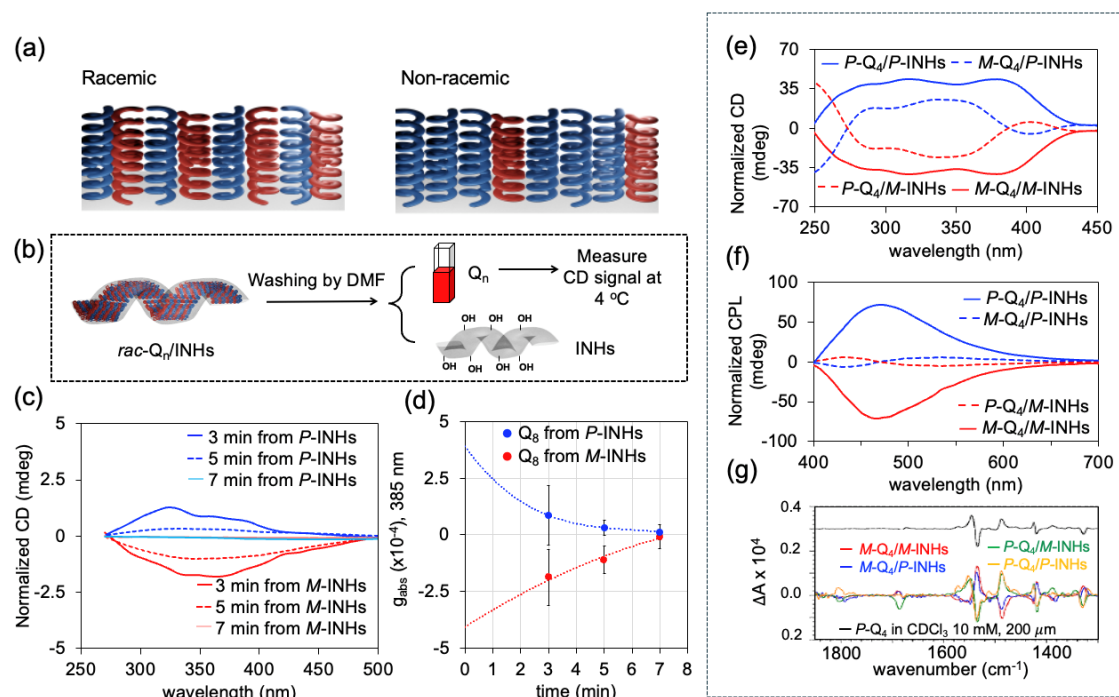
Fig. 4 (a) Illustration of two possibilities after drop-casting rac - Q_n on INHs corresponding to the relation between g_{abs} and foldamers. (b) Recovering of Q_8 from INHs by simple washing with an organic solvent. (c) ECD spectra of rac - Q_8 in DMF after removing from INHs (average from 20-time experiment), (d) Plot between g_{abs} of rac - Q_8 (at 385 nm) in function of time with the standard deviation. (e) ECD-absorption, and (f) CPL-fluorescence spectra of M - Q_4 /INHs and P - Q_4 /INHs ( \lambda_{ex} = 320 nm). (g) (top) VCD spectrum of P - Q_4 foldamer in CDCl_3 solution (10 mM, 200 \mu m pathlength). (bottom) Normalized differential VCD spectra of M - Q_4 / M -INHs, M - Q_4 / P -INHs, P - Q_4 / M -INHs and P - Q_4 / P -INHs samples after subtracting corresponding rac - Q_4 / P or M -INHs.
