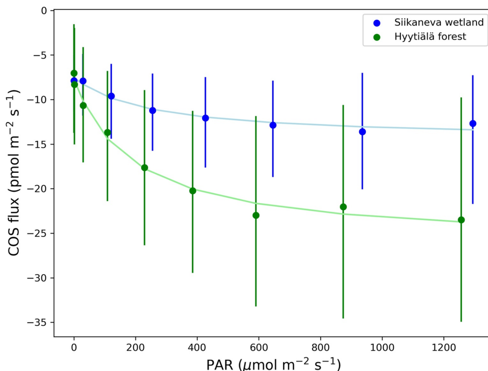
Figure 2. Carbonyl sulfide flux relationship with photosynthetically active radiation (PAR). Siikaneva wetland in blue and Hyytiälä forest data in green. Data is collected in 10 equally sized bins. Error bars represent 25 and 75 percentiles. Regression equations: y = ((-6.9 \cdot \text{PAR}) / (\text{PAR} + 241)) - 7.5 for the wetland and y = ((-19 \cdot \text{PAR}) / (\text{PAR} + 190)) - 7.6 for the forest.
