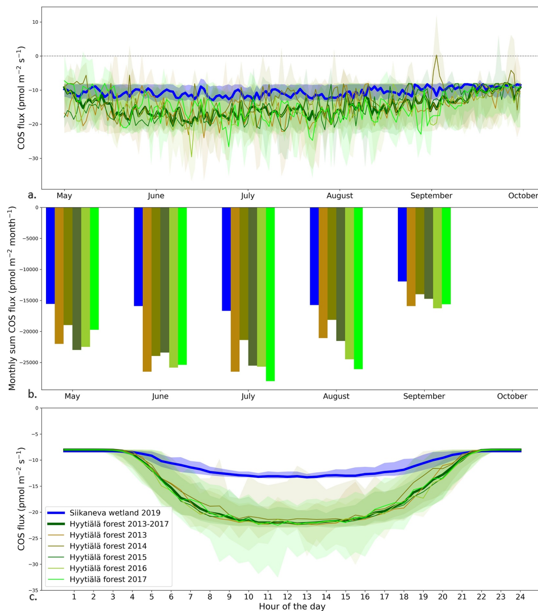
Figure 1. (a) Daily median gap-filled carbonyl sulfide (COS) fluxes with 25 and 75 percentiles. (b) Monthly sums of gap-filled COS fluxes. (c) Mean diurnal cycle of gap-filled COS flux with 25 and 75 percentiles. Blue for Siikaneva wetland and green variations for Hyytiälä forest. COS sink reported as negative flux.
