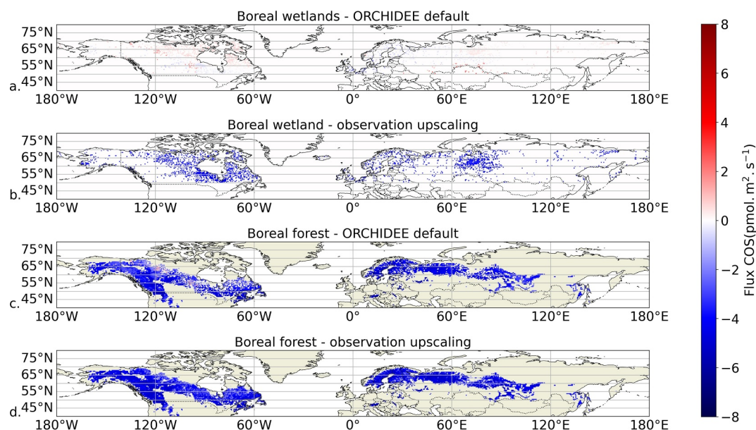
Figure 3. Organizing Carbon and Hydrology In Dynamic Ecosystems (ORCHIDEE) simulations. In (a, c) the default boreal ORCHIDEE output for the wetland/forest carbonyl sulfide (COS) fluxes and in panels (b, d) the fluxes calculated based on the measured median wetland/forest COS flux.
