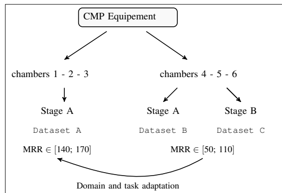
Fig. 2: Tree representation of PHM dataset
