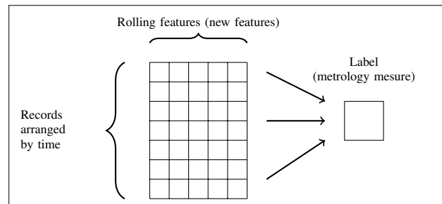
Fig. 1: 2D Input representation of FDC raw data
