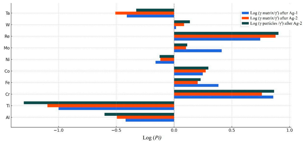
Figure 10. Partitioning behavior of elements between the FCC \gamma matrix and the L1 2 \gamma' phase, as well as between \gamma particles and the \gamma' phase, in the HESA-X1 alloy after Ag-1 and Ag-2 heat treatments.
