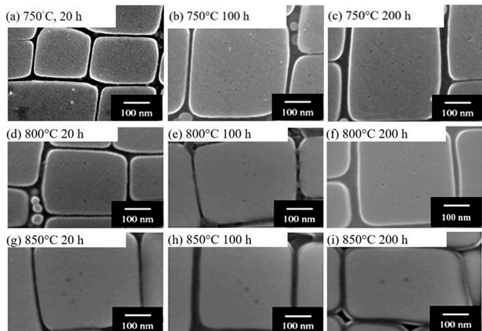
Figure 11. SEM observations of HESA-X1 alloys are exposure at 750 °C, 800 °C, and 850 °C from 20, 100, and 200 h after Ag-2 aging heat treatment.
