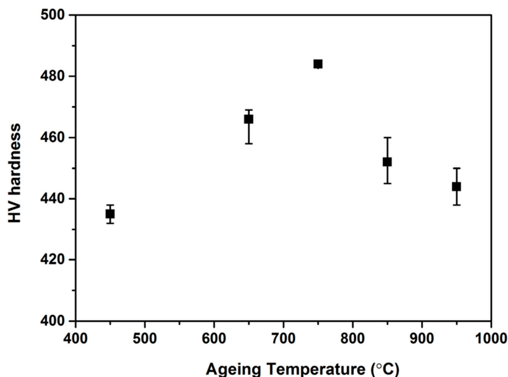
Figure 6. Vickers hardness of the HESA-X1 alloy as a function of aging temperature after Ag-1 treatment. All aging treatments were conducted for 20 h.
