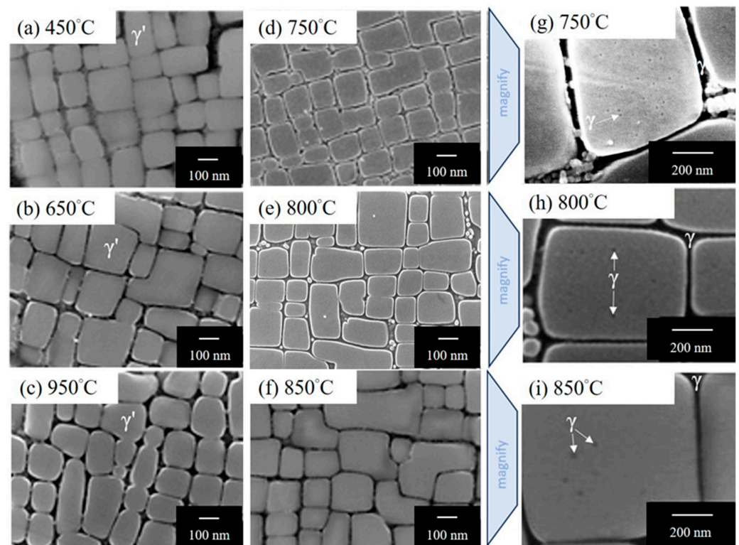
Figure 5. SEM images of the evolution of \gamma' morphology in the HESA-X1 under various aging temperatures for 20 h. (a–f) represent the general \gamma/\gamma' microstructure at different temperatures: (a) 450 °C, (b) 650 °C, (c) 950 °C, (d) 750 °C, (e) 800 °C, and (f) 850 °C. (g–i) are magnified views of \gamma' precipitates within the \gamma matrix from (d–f), highlighting the formation of \gamma particles within the \gamma' phase for (g) 750 °C, (h) 800 °C, and (i) 850 °C.
