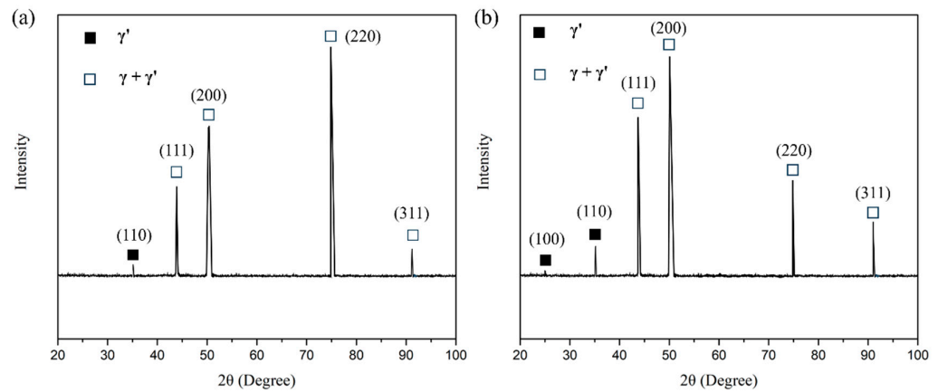
Figure 12. XRD patterns of the HESA-X1 alloy showing \gamma' and \gamma + \gamma' phases: (a) as-cast condition and (b) after Ag-2 treatment followed by additional aging at 850 °C for 200 h. The diffraction peaks correspond to the \gamma' phase (solid squares) and overlapping \gamma + \gamma' phases (open squares).
