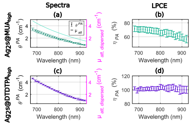
Figure 3: Photoacoustic and attenuation spectra ((a) and (c)) and Light-to-Photoacoustic Conversion Efficiency (LPCE, (b) and (d)) for the silver sulfide (Ag 2 S) prepared with a high concentration of AgNO 3 and with two different coatings: Ag 2 S@MUA high and Ag 2 S@DTDTPA high , respectively. The photoacoustic coefficients \theta^{PA} were obtained with a calibrated photoacoustic spectrometer. Here, \theta^{PA} is assumed to be equal to the photothermal conversion efficiency multiplied by the absorption coefficient of the dispersed phase. The attenuation coefficient \mu_{att, dispersed}(\lambda) is measured with a spectrophotometer. The LPCE is the ratio of \theta^{PA} to \mu_{att, dispersed}(\lambda) . For the photoacoustic coefficients, the median \pm median absolute deviation values were displayed with dot markers and error bars. For the LPCE, the error bars correspond to the relative uncertainty and consider all the measurement and calibration steps. The axis ranges for the LPCE were 40%.
