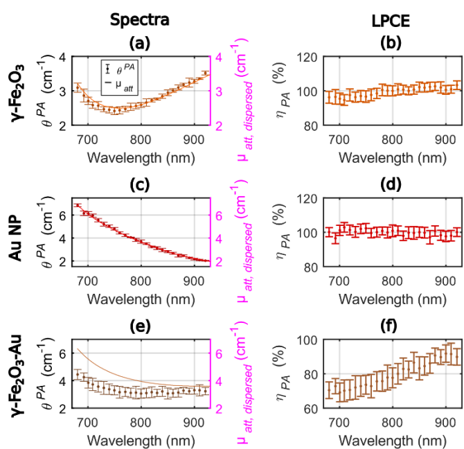
Figure 4 Photoacoustic and attenuation spectra ((a), (c) and (e)) and Light-to-Photoacoustic Conversion Efficiency (LPCE, (b), (d) and (f)) for the maghemite nanoflowers ( \gamma\text{-Fe}_2\text{O}_3 ), the gold nanoparticles (Au NP) and the maghemite nanoflowers decorated with gold nanoparticles ( \gamma\text{-Fe}_2\text{O}_3\text{-Au} ), respectively. The photoacoustic coefficients \theta^{PA} were obtained with a calibrated photoacoustic spectrometer. Here, \theta^{PA} is assumed to be equal to the photothermal conversion efficiency multiplied by the absorption coefficient of the dispersed phase. The attenuation coefficient \mu_{att,dispersed}(\lambda) is measured with a spectrophotometer. The LPCE is the ratio of \theta^{PA} to \mu_{att,dispersed}(\lambda) . For the photoacoustic coefficients, the median \pm median absolute deviation values were displayed with dot markers and error bars. For the LPCE, the error bars correspond to the relative uncertainty and consider all the measurement and calibration steps. The axis ranges for the LPCE were 40%.
