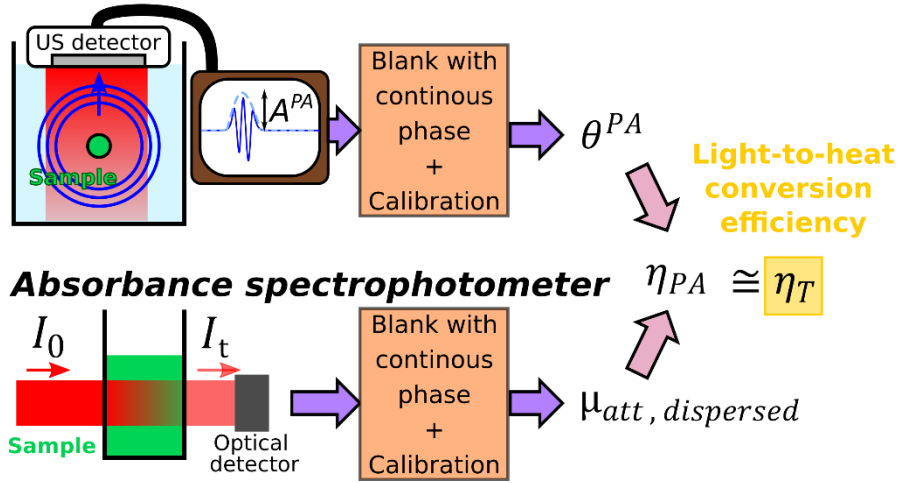
Figure 1: Experimental method proposed for the determination of the light-to-heat conversion efficiency using photoacoustic spectrometry and absorbance spectrophotometry of a given aqueous suspension of nanoparticles. For the photoacoustic spectrometer, the sample is placed in a tube and illuminated with pulsed light. The amplitude of the ultrasound (US) wave generated with the photoacoustic effect is measured from the signal captured with an US detector. This ultrasound amplitude is converted in the photoacoustic coefficient \theta^{PA} thanks to a calibration process. For the absorbance spectrophotometer, the sample is placed in a cuvette of known path length and illuminated by continuous light. The ratio of the transmitted light power and the incident light power measures the transmittance, that can be converted in the attenuation coefficient. Both spectrometers are blanked with the continuous phase, this leads to obtain coefficients for the dispersed phase. The light-to-photoacoustic conversion efficiency \eta_{pa} is then obtained from the ratio between the photoacoustic coefficient and the attenuation coefficient. When the Grüneisen coefficient of the solution can be assumed to be the Grüneisen coefficient of water, \eta_{pa} equals \eta_T the light-to-heat conversion efficiency, LHCE.
