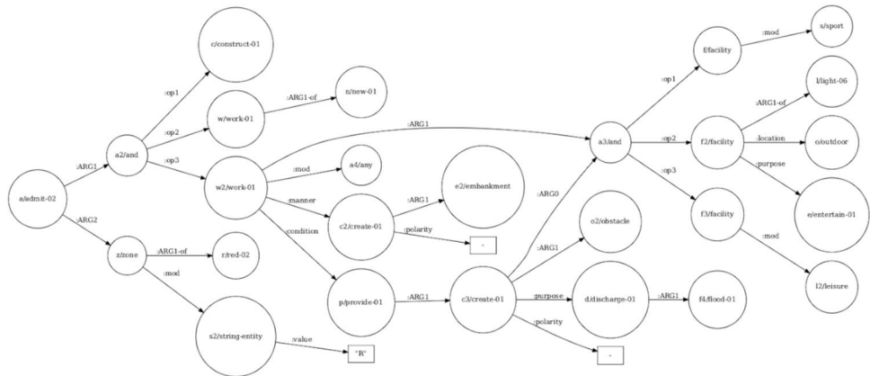
Subgraph 1 corresponding to the keyword «CONSTRUCTIONS» (associated word in English is «construct»):
