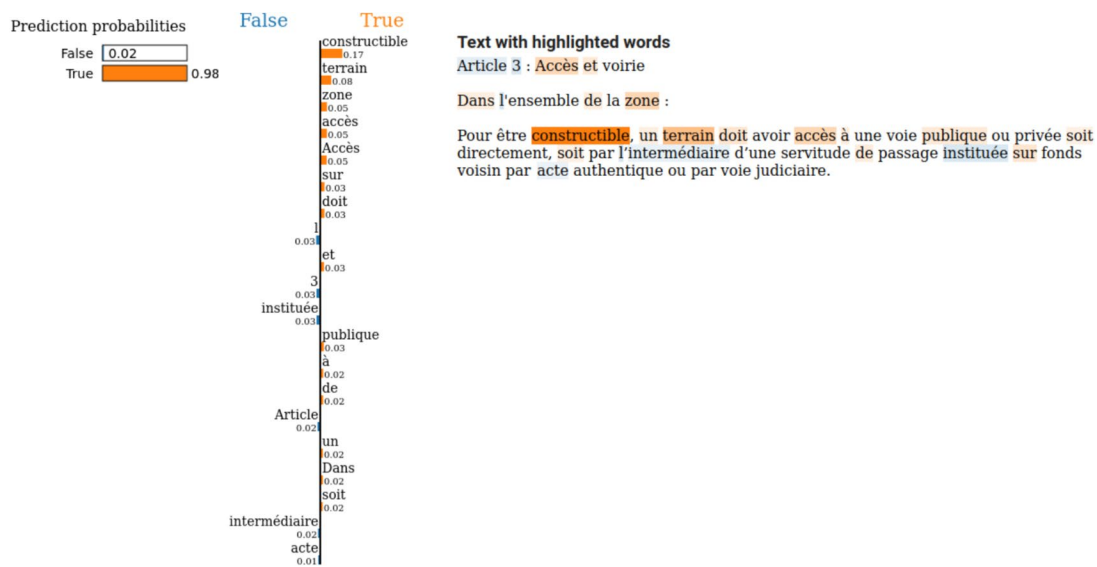
Fig. 13 An example of a segment analysis using Lime, from left to right: the classification results with probability scores, the features which led to these results, original segment with negative and posi-
