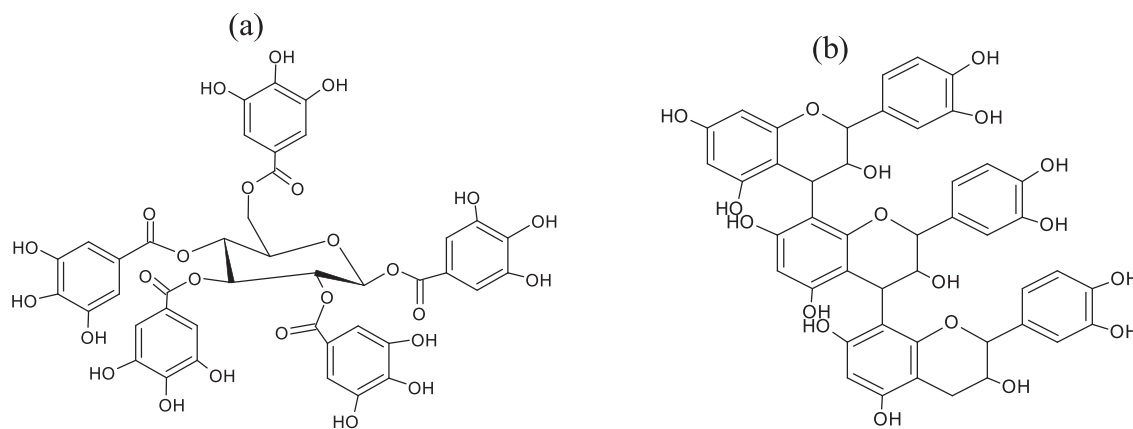
Figure 6.—Structures of hydrolysable tannin (a), condensed tannin (b).
