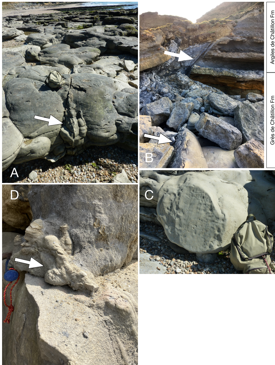
Figure 3. Structures pictured at the Cran du Noirda (see Figure 1) accompanying the synsedimentary fault movement. (A) Indurated injectites visible on the cemented nodules. (B) The fault plane itself, also visible in Figure 1), affecting the transition zone between the Grès de Châtillon and Argiles de Châtillon formations. The fault cut some sandstone nodules (lower arrow in B, C). (D) A soft sand injective penetrating the Argile de Châtillon Fm.
