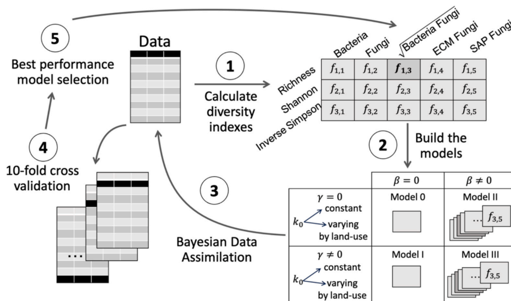
Fig. 2. Illustration of the 5-step process for model selection based on diversity indices and Bayesian data assimilation: (1) Raw data (i.e., microbial functional groups such as bacteria, fungi, combined fungi and bacteria, ectomycorrhizal (ECM) fungi, and saprotrophic (SAP) fungi) are used to compute various diversity indices (i.e., Richness, Shannon, and Inverse Simpson), resulting in a total of 15 microbial diversity indices; (2) different models are constructed based on varying assumptions about the influence of microbial biomass ( \gamma \neq 0 in Eq. (2)) and microbial diversity ( \beta \neq 0 Eq. (6)) on heterotrophic respiration and net N mineralization rates. Models including the effect of microbial diversity (i.e., models II and III) were built for each of the 15 diversity indices (denoted here f_{i,j} , with i = 1, \dots, 3 and j = 1, \dots, 5 ), resulting in a total of 32 models; (3) model parameter probability distributions are estimated via a Bayesian data assimilation framework to predict heterotrophic respiration and net N mineralization. Two calibration strategies are carried out, one with constant decay rate coefficient k_0 , and one with k_0 varying by land-use; (4) the models undergo a 10-fold cross-validation, where the dataset is split into 10 subsets and the models' performance is tested iteratively on the different subsets; (5) finally, the best performance models are selected based on the average cross-validation results.
