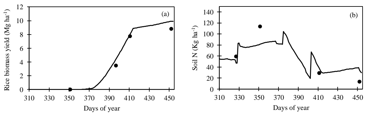
Figure 1: Comparison of observed and STICS simulated rice biomass (a) and soil N (b) dynamics during rice growing cycle for rice residues with manure and mineral fertilizer (160 kg N ha -1 )
