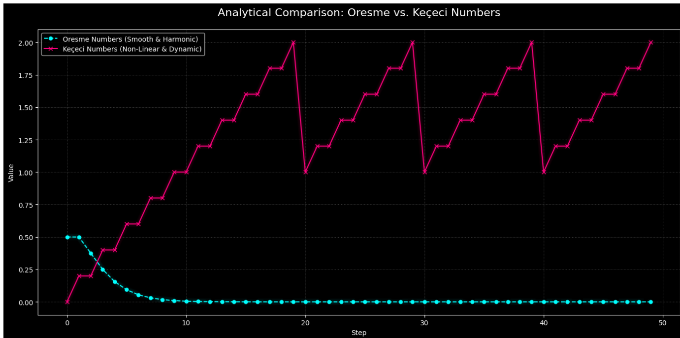
Figure 8: Analytical Comparison Oresme vs. Keçeci Numbers
