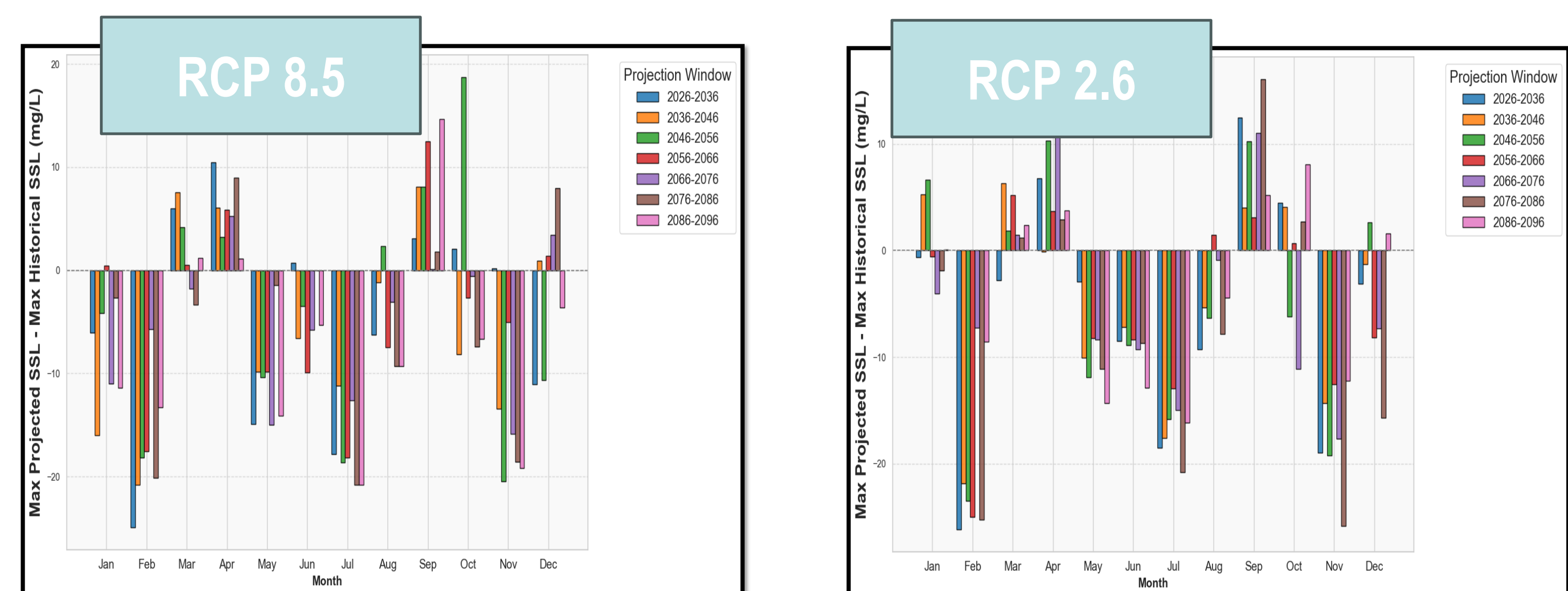
Figure 6: Maximum difference between historical and projected SSL across two scenarios
