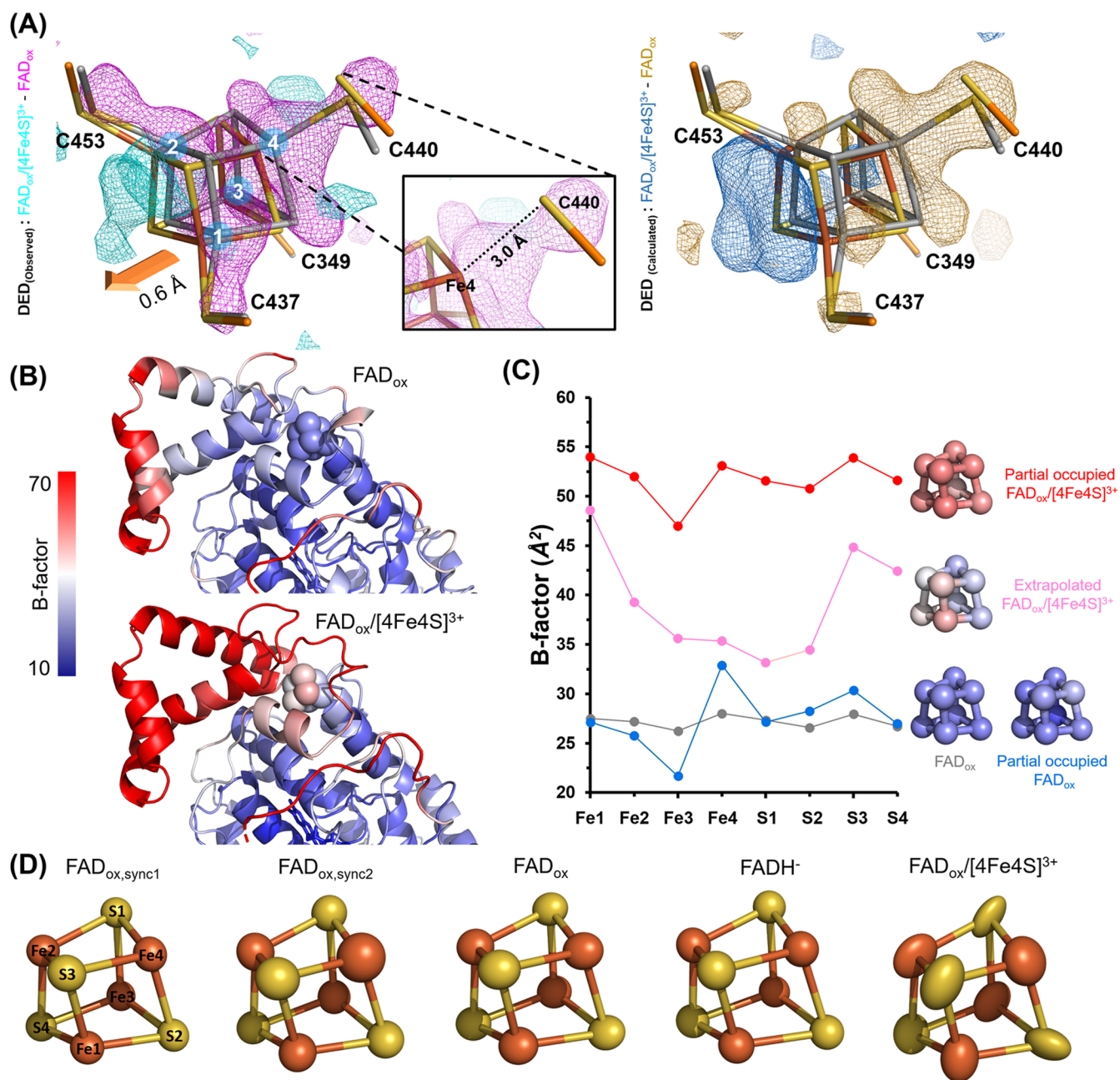
Figure 6. Structural changes in iron–sulfur cluster between FAD_{ox} and FAD_{ox}/[4Fe-4S]^{3+} states. (A) Structural changes in the [4Fe-4S] cluster upon its oxidation. The [4Fe-4S] cluster shifts by \sim 0.6 Å toward the solvent (arrow, orange), whereas the components of [4Fe-4S] exhibit complete covering of negative density. The FAD_{ox}/[4Fe-4S]^{3+} state of Cc (6–4)PL (orange) is shown in comparison of FAD_{ox} (gray). For highlighting the significance of observed differences, 3.5\sigma contoured DED maps are shown in cyan and magenta for positive/negative peaks. For calculated differences, 3.5\sigma contoured DED maps are likewise shown in blue and gold for positive/negative peaks. The map correlation between observed DED maps (left) and calculated ones (right) is shown to be high; the map correlation value is listed in Table S2. The inset shows atom–atom distances in Angstrom. (B) B-factor distribution around the roof-like domain. Oxidation of the [4Fe-4S] cluster to the +3 state causes increased B-factors for regions of the roof-like domain, which are well ordered in the +2 state. (C) B-factor plots and CPK models of the [4Fe-4S] cluster in its +2 and +3 states. Oxidation toward the FAD_{ox}/[4Fe-4S]^{3+} state (pink, from extrapolated data) causes increased thermal mobility when compared with the FAD_{ox} state (gray). Increased disorder of the [4Fe-4S]^{3+} cluster can be also delineated from B-factor distributions, when performing instead partial-occupancy refinement of both the FAD_{ox}/[4Fe-4S]^{2+} (66% occupancy, blue) and FAD_{ox}/[4Fe-4S]^{3+} (34%, red) states against nonextrapolated FAD_{ox}/[4Fe-4S]^{3+} SFX data. (D) Anisotropic B-factor refinement of the [4Fe-4S] cluster. The anisotropic thermal motion of each atom on [4Fe-4S] at redox states was depicted as ellipsoids.
