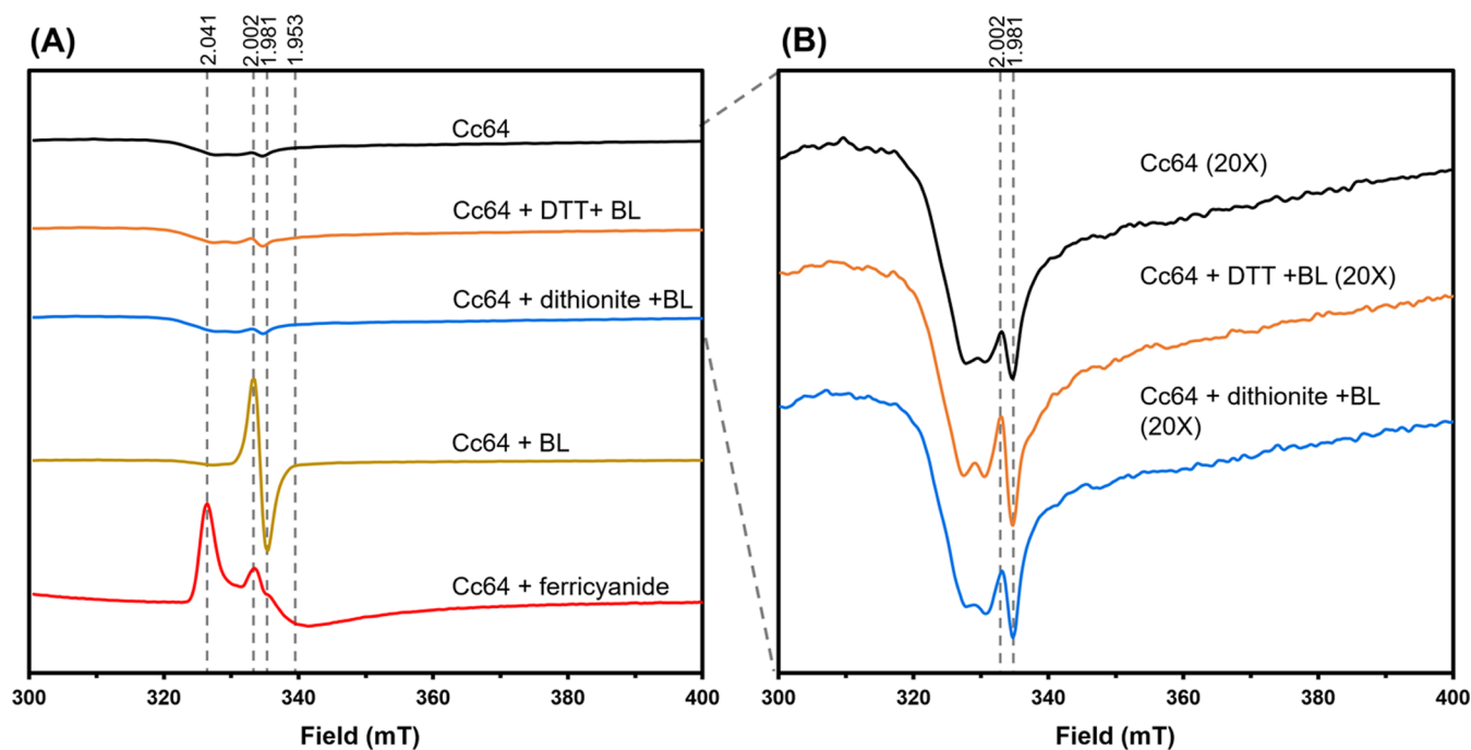
Figure 1. X-band EPR spectra of different redox states of Cc (6–4)PL at 10 K. (A) Coloring of the EPR signals with Cc (6–4)PL (black), with 50 mM DTT (orange), with 2 mM dithionite (blue), with 455 nm blue light (BL) for 30 min (gold), and 2 mM ferricyanide for 3 min (red). (B) Close view of EPR-silent samples. EPR conditions: microwave power, 0.2 mW; modulation amplitude, 1.0 mT; modulation frequency, 9.35 kHz. Treatment of Cc (6–4)PL with ferricyanide did not affect the EPR-silent oxidized state of the FAD chromophore, as also shown by UV/vis data (Figure S4A).
