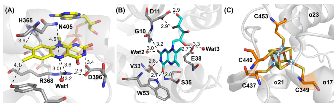
Figure 3. Cofactors' interaction sites within the damage-free structure of oxidized Cc (6–4)PL. (A) FAD binding pocket with surrounding residues (gray sticks) and waters (red spheres). A water molecule, Wat1, forms a hydrogen bond with the N5 atom of the isoalloxazine ring; corresponding atom–atom distances are given in Angstrom (Å). (B) DLZ binding site, with nearby residues (gray) and water molecules (red), which are involved in hydrogen-bonding networks between the chromophore and the protein. (C) Binding site for the [4\text{Fe-4S}]^{2+} cluster in its C-terminal roof-like subdomain. The conserved four cysteines are shown as stick models as well as the [4\text{Fe-4S}] cluster with its numbered iron atoms.
