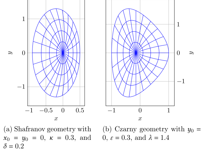
Fig. 2. Two geometries are considered.
