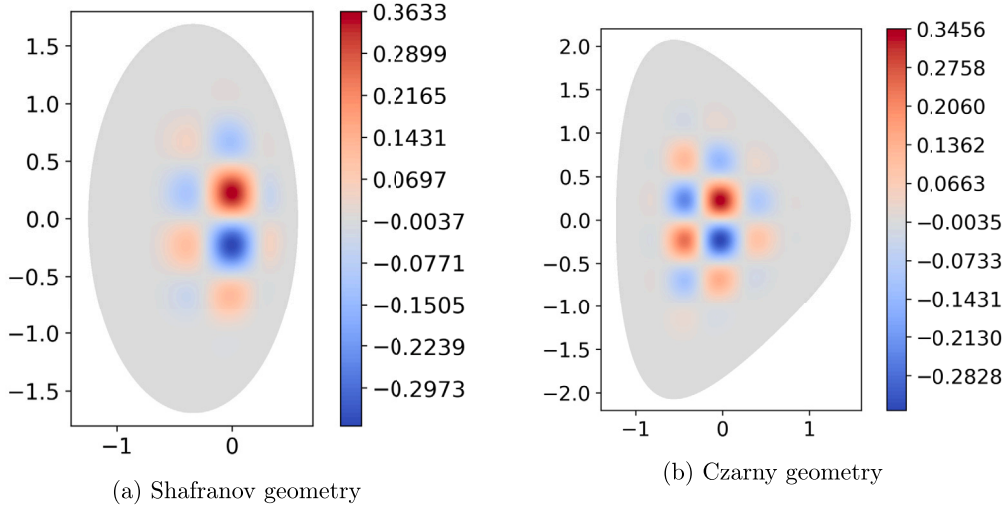
Fig. 9. Illustration of the manufactured solution (60) for the Shafranov and Czarny geometries.
