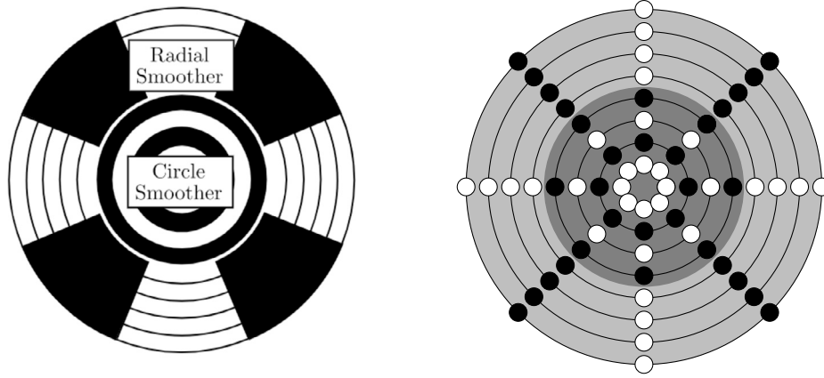
Fig. 3. Left: Schematic subdivision of a circular domain into an interior subdomain where circle-line smoothing is used and an exterior subdomain where radial smoothing is used. Right: Circular mesh with 64 nodes. Circular smoothing applied on the four interior circles (dark gray background color), radial smoothing applied on the four exterior circles (light gray background color). Nodes colored according to smoother color.
