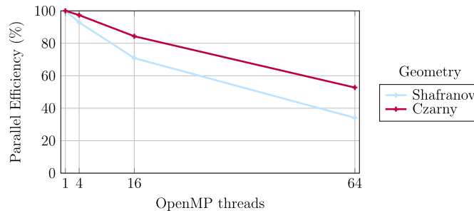
Fig. 12. Weak scaling of GMGPolar. Parallel efficiency compared to the sequential run from 1 to 64 cores on grids of size 769 \times 1024 to 6145 \times 8192 , manufactured Cartesian solution (60).
