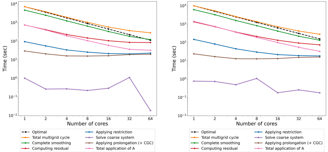
Fig. 13. Strong scaling of GMGPolar. From 1 to 64 cores on a grid of size 6145 \times 8192 , Shafranov geometry Fig. 2a (left) and Czarny geometry Fig. 2b (right) and manufactured solution (60).
