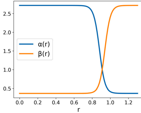
Fig. 10. Coefficients \alpha and \beta used in Equation (1).
