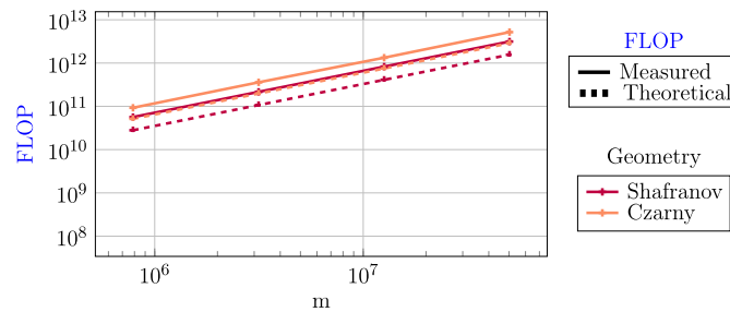
Fig. 11. Computational cost in FLOP when applying GMGPolar for the manufactured Cartesian solution (60) on the geometries Shafranov and Czarny. We include the number of flops as measured by LIKWID as well as the theoretical (asymptotic) expectations.
