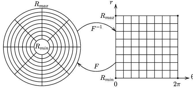
Fig. 1. A circular geometry described (Left) in Cartesian coordinates and (Right) in polar coordinates (r, \theta) \in [R_{min}, R_{max}] \times [0, 2\pi) with mappings F and F^{-1} between the different descriptions.
