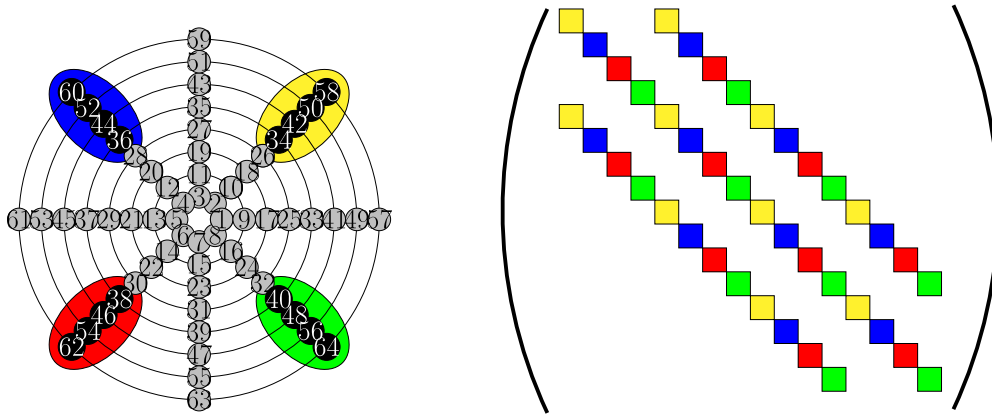
Fig. 4. Left: Circular mesh with 64 nodes as in Fig. 3 (right). Without loss of generality, we assume a circle-wise global numbering. Focus on black colored nodes of the radial smoother. Different grid lines of the smoother given by different background colors. Right: Nonzero pattern of the submatrix A_{R_B R_B} when using a compact five, seven, or nine point stencil, with colors referring to the particular grid lines as depicted on the left figure. Different numberings of the nodes lead to different nonzero patterns.
