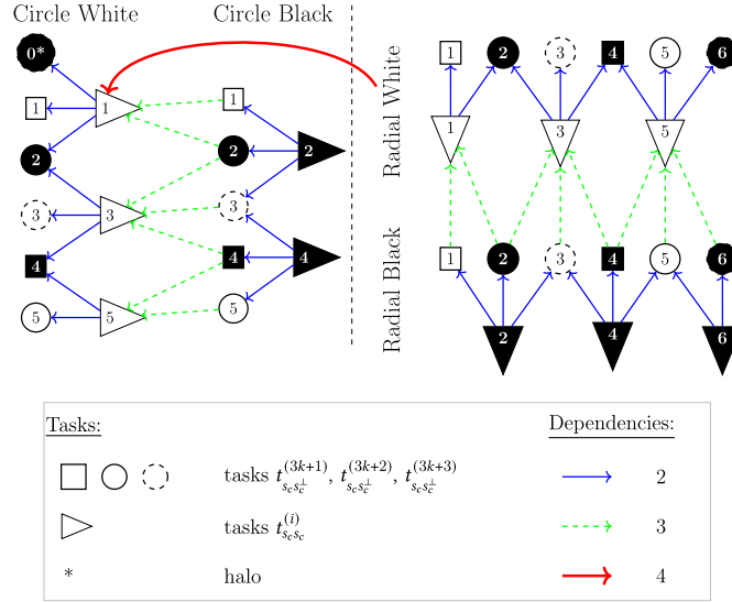
Fig. 8. Dependency graph for the application of the smoother. Each node is a task, i.e., the handling of a circle line of nodes. The tasks t_{s_c, s_c^\perp}^{(i)} , i = 2, 3, 5 and i = 2, 3, 5, 6 , are represented by circles and tasks t_{s_c, s_c^\perp}^{(i)} , i = 1, 4 are squares. Tasks t_{s_c, s_c}^{(i)} , i = 1, 2, \dots , are represented by triangles. The different type of dependencies are colored: 2 = blue, 3 = green, and 4 = red. For the sake of a simple presentation, we do not display the dependencies from (56), as they are identical to what is shown in Fig. 7.
