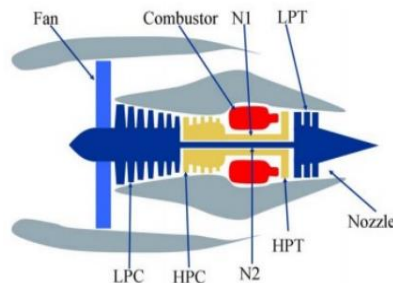
Figure 2. Simplified diagram of a simulated turbojet in C-MAPSS
