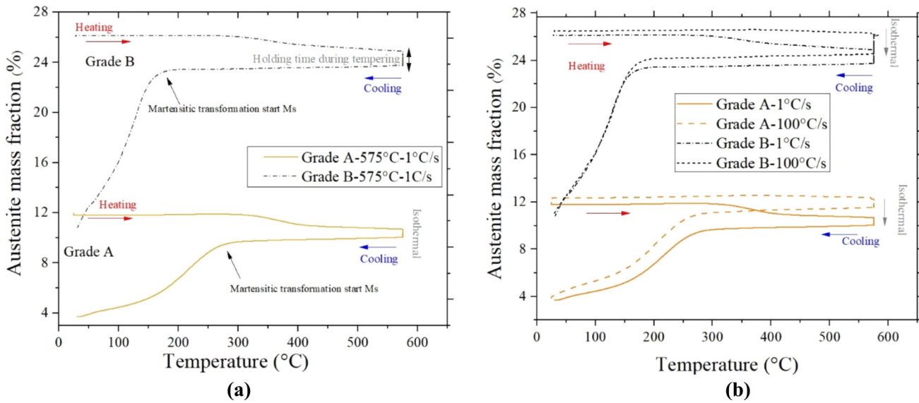
Fig. 5—Comparison of the evolution of the retained austenite mass fractions measured by HEXRD of both grades A and B; (a) evolution of the retained austenite mass fraction as a function of temperature at a heating rate of 1 °C/s, (b) influence of the heating rate on the retained austenite mass fraction variation as a function of temperature.
