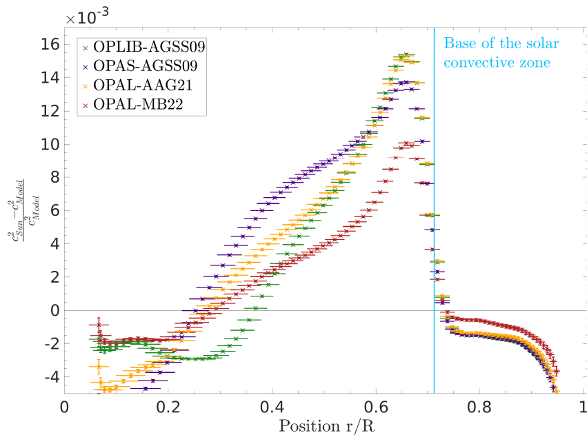
Figure 3. Relative differences in squared adiabatic sound speed for models built with various abundances and opacity tables (namely AAG21, AGSS09 and MB22 for abundances and OPAS, OPLIB and OPAL for opacities).
