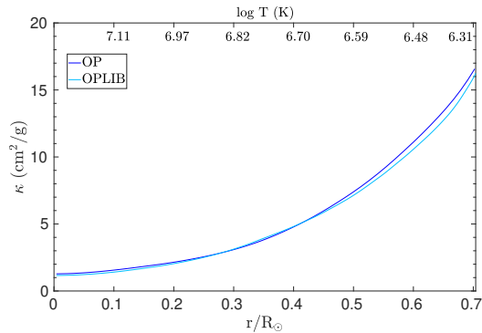
Figure 1. Comparison between the OP and OPLIB opacities in the solar radiative zone, on the same thermodynamical coordinates ( \rho , T , X , Z ).
