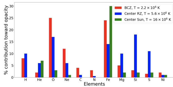
Figure 2. Contribution of chemical various elements to the Rosseland mean opacity in three characteristic regions of the radiative interior of the Sun.
