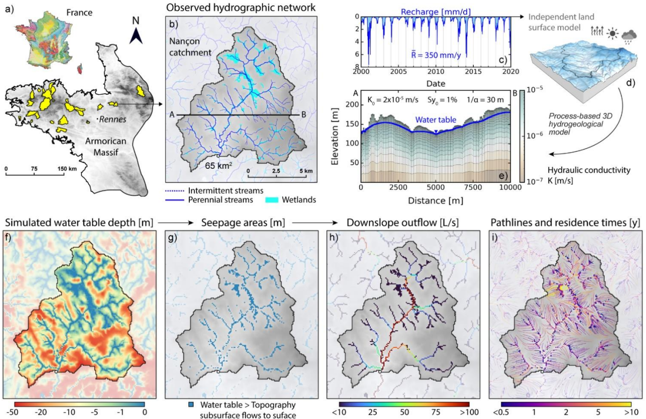
210 Figure 2. HydroModPy modeling steps illustrated on the site of Nançon. (a) Extraction of the watershed from a regional DEM. (b) Clip data based on the watershed extent. (c) Recharge time series provide from an independent land surface model. (d) 3D diagram illustrating the model conceptualization and parameterization based on data and assumptions. (e) The cross-section (A-B) illustrates the vertical grid discretization and the resulting water table. The parameters include an exponential decay of 1/\alpha (m) with depth 215 from the maximum hydraulic conductivity K_0 and specific yield Sy_0 (%) in the first layer. (f-i) 2D map view visualization displaying spatial data and model results in steady state across the study area (left to right): watertable depth, seepage areas, accumulated outflow, pathlines and residence times.
