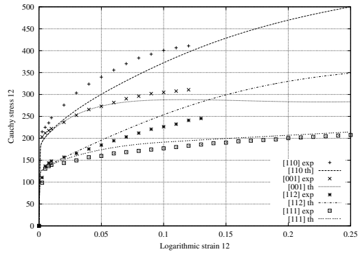
Fig. 1. Single crystals shear tests
