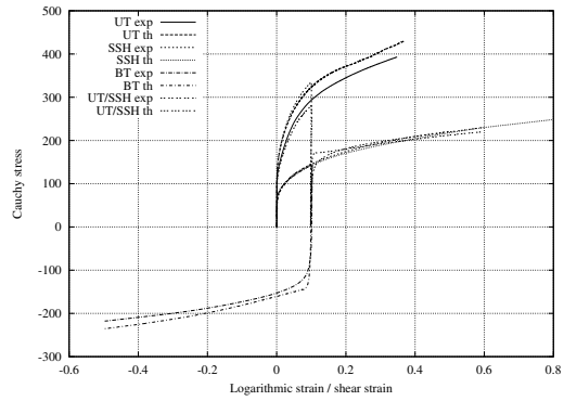
Fig. 2. Polycrystal behavior prediction
