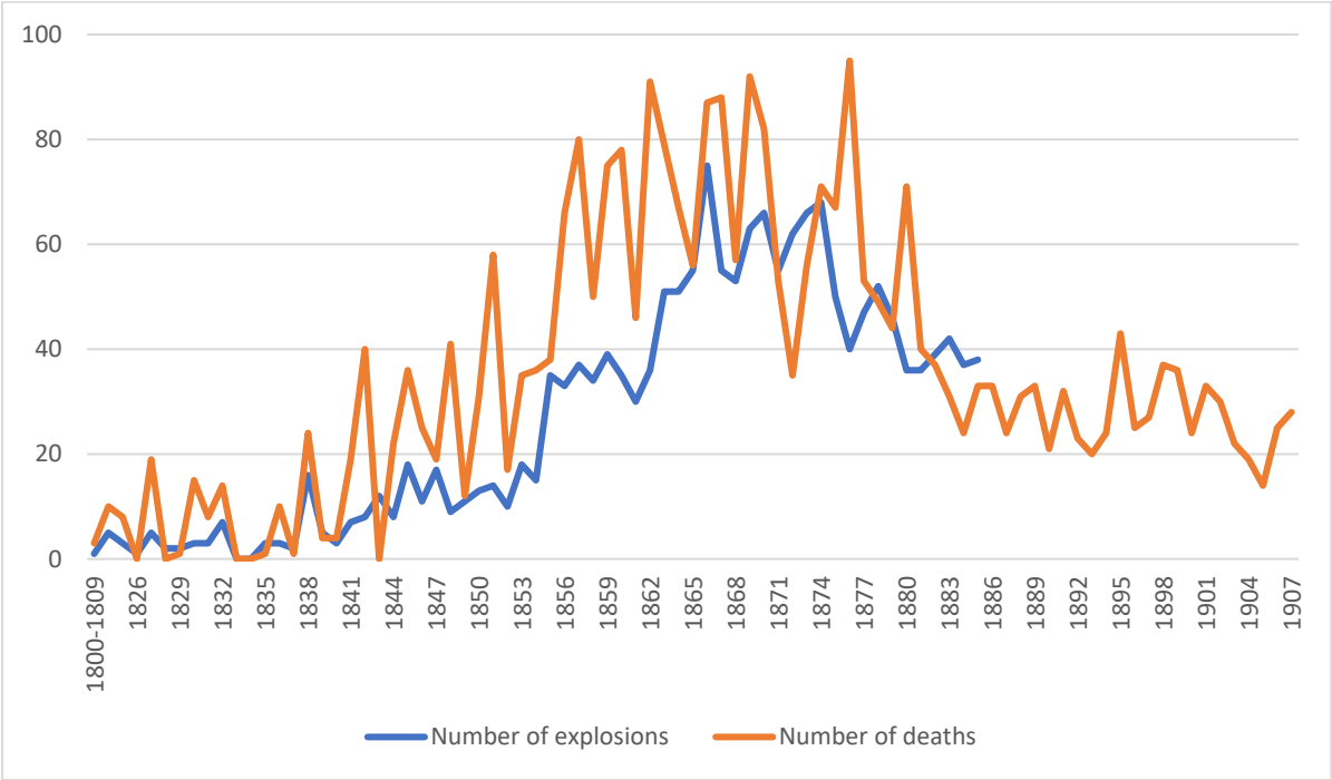
Figure 1. The number of explosions and casualties from steam boiler explosions in Britain began to decline in the 1870s with the spread of regular inspections by insurance companies
