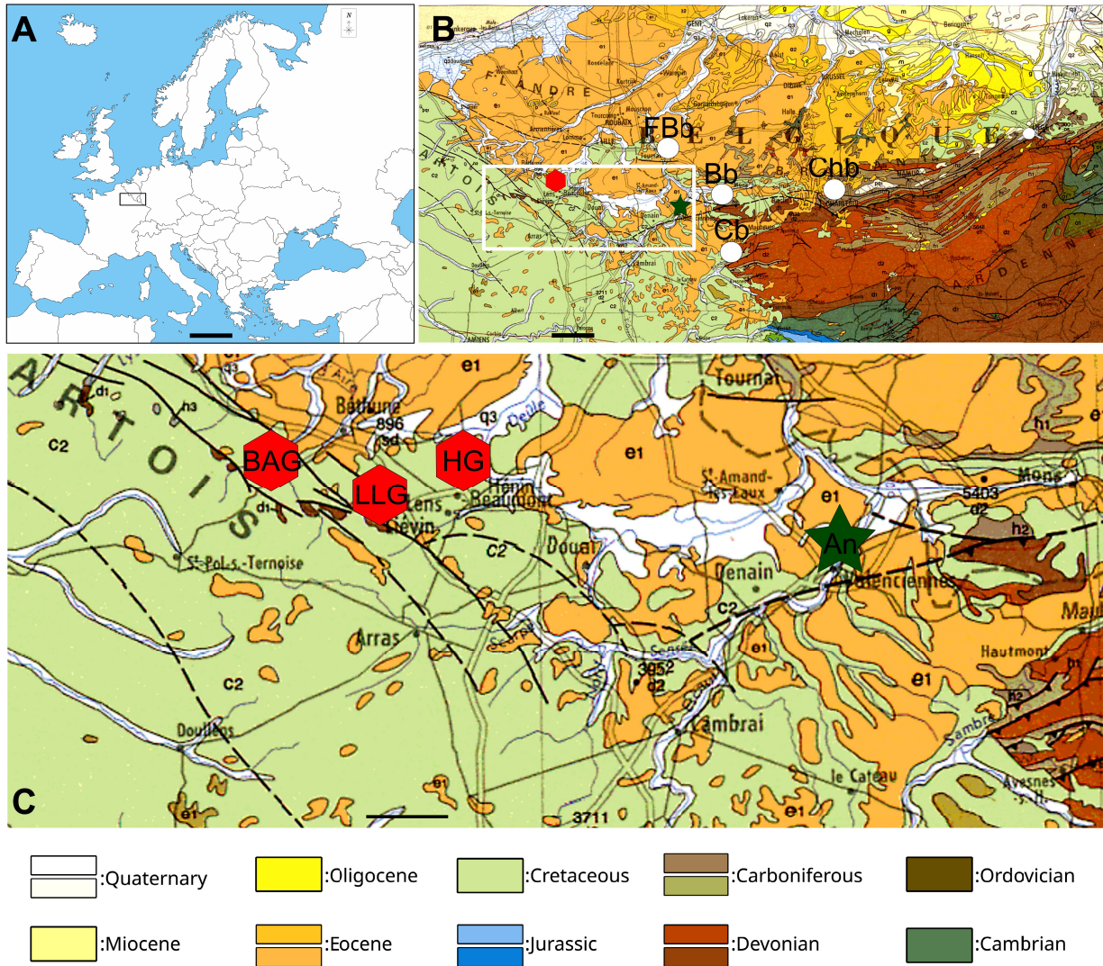
Figure 1. Location of the studied material. A: position of the French and Belgian coalfields. B: position of the Pas-de-Calais basin, where the 'ancient material' (Pruvost, 1919, Anzin Formation, Westphalian B i.e. Baskirian-Moscovian, green star) and the new specimens from the Bruay Formation (Westphalian C i.e. Moscovian, red hexagon) were found. C: details of the position of the Bruay Formation in the Pas-de-Calais basin. The Bruay specimens come from three different zones exploited by different mining companies: the Bruay-Auchel Group (BAG), the Lens-Liévin Group (LLG) and the Hémin Group (HG). Note that the coalfields are not visible on the map at this scale, being covered by Cretaceous sediments and located in underground mines. An, Anzin; Bb, Borinage basin; Cb, Center basin; Chb, Charleroi basin; FBb, Franco Belgian basin. Scale bars = 10 km (B, C), 500 km (A). Vectorised map in A from © d-maps.com.
