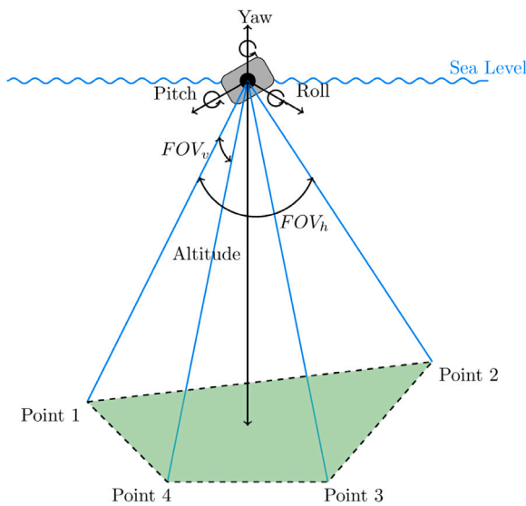
Fig. 8. Footprint calculation of underwater images based on echosounder data, camera field of view and ASV angles.
