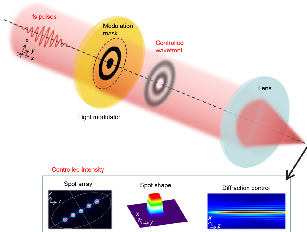
Fig. 1 | Principle of spatial beam shaping of ultrafast laser. A light modulator (transmittive or reflective) is placed on the laser beam path. It imprints a wavefront modulation (modulation mask) that rearranges the laser intensity distribution in a further plane of propagation, usually the focal plane of a converging element. There, a variety of beam distributions can be obtained in he three dimensions, from multi-spot arrangement to continuous beam shapes, as well as non-diffracting beams.
