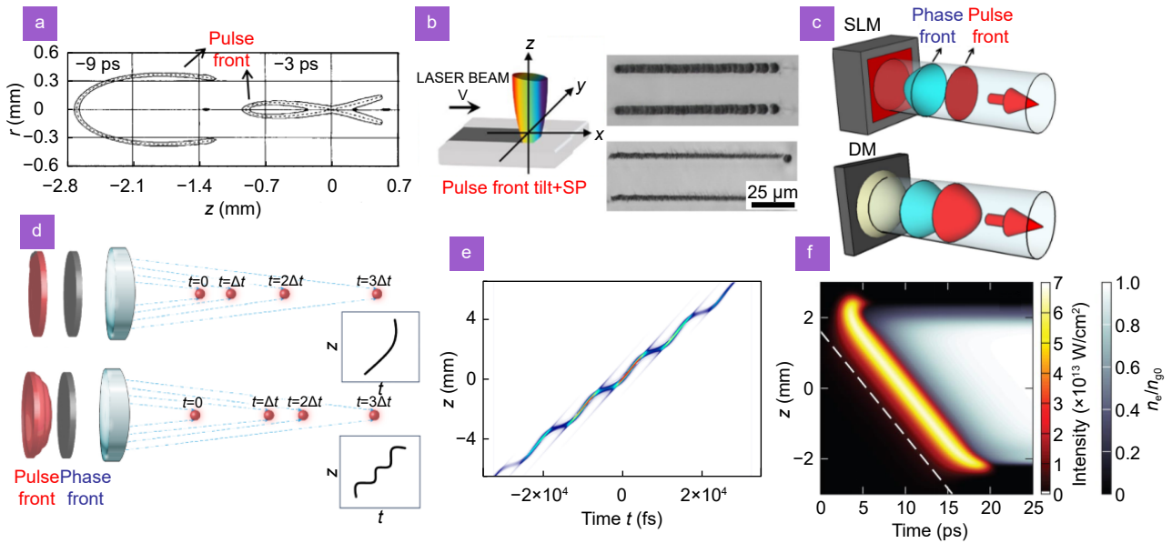
Fig. 10 | Future research trends taking advantage of the temporal effects associated with spatial shaping. (a) Illustration of the pulse front distortion around the focal point implying complex consequences on the spatial and temporal properties of the local excitation. (b) Pulse front tilt and spatial chirp involving non reciprocal photo inscription on glasses. (c) Concepts for pulse front and wavefront modulation based on an SLM and a DM. (d) Controlling the velocity of the intensity focal point in the focal region along z by tuning the pulse and phase fronts. (e) Simulation of a controlled intensity trajectory with accelerating and decelerating steps. (f) Overcoming ionization induced refraction by controlling the flying focus speed. Figure reproduced with permission from: (a) ref. 259 , Springer Nature; (b) ref. 260 , under a Creative Commons Attribution License; (c) ref. 261 , the author; (d) ref. 262 , under the Optica Open Access Publishing Agreement; (e) ref. 263 , the author; (f) ref. 264 , the author.
