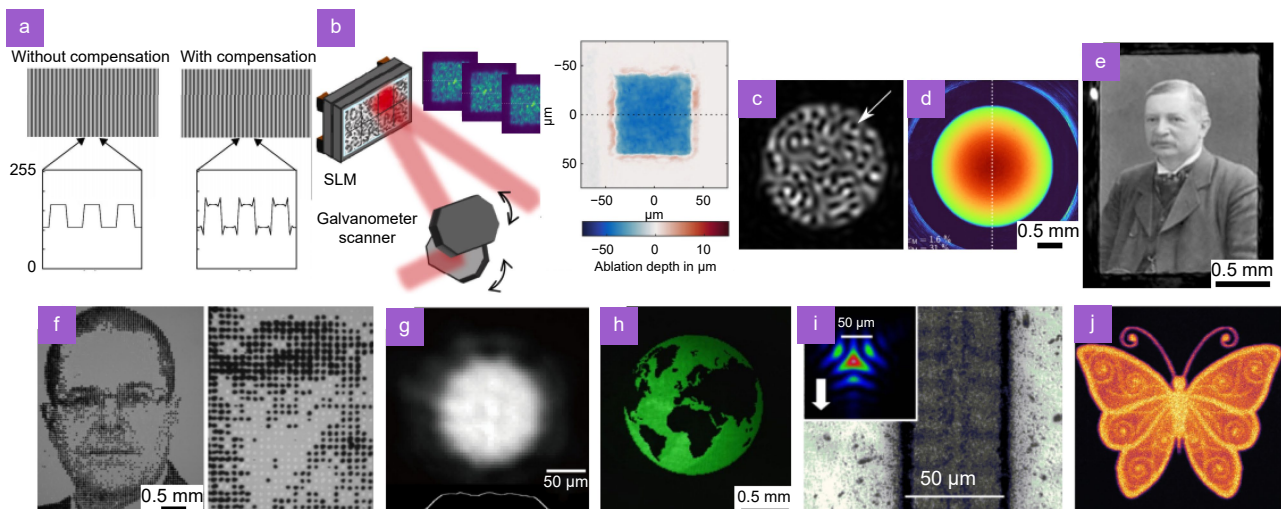
Fig. 9 | Examples of recently developed to improve the fidelity and/or efficacy of spatial beam shaping. (a) Compensating the limited spatial resolution of SLM by using spatial frequency filtering of the phase modulation. (b) Averaging the detrimental speckle effect by addressing different phase masks on the SLM for uniform multi-pulse ablation. (c) Incorporating Vortex elimination during the phase modulation calculation step. (d, e) High fidelity intensity distribution shaping in the region of interest with the compromise of energy losses for atom trapping. (f) Parallel surface structuring using multi-spot arrays with individually controlled spot intensity based on an optical feedback of the experimental intensity distribution. (g) Smooth top hat generation using optical feedback to adjust the intensity pattern in the iterative Fourier transform algorithm. (h) Arbitrary intensity distribution using the GPC technique. (i) Groove machining with controlled intensity distribution using Zernike polynomials optimization. (j) Spatial beam shaping based on diffractive optical neural network. Figure reproduced with permission from: (a) ref. 200 , the author; (b) ref. 201 , under a Creative Commons Attribution License; (c) ref. 118 , Optical Society of America; (d) ref. 202 , (e) ref. 92 , under a Creative Commons Attribution License; (f) ref. 90,92 , Optical Society of America; (g) ref. 203 , the author; (h) ref. 65,68 , the author; (i) ref. 204 , Optical Society of America; (j) ref. 226 , under Optica Open Access Publishing Agreement.
