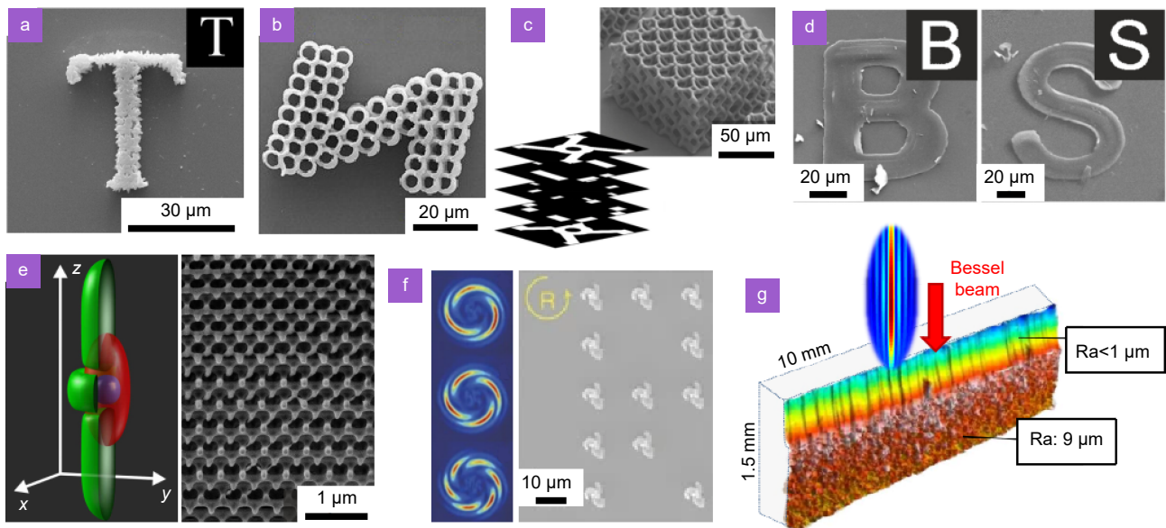
Fig. 8 | Additive fabrication using spatial beam shaping. Two photon polymerization using arbitrary beam shapes (a) and an array of laser spots (b). (c) Continuous projection of femtosecond pulses using digital micro-mirror device with spatio temporal focusing permits high throughput photo polymerization. (d) Laser induced forward transfer of polymer on PDMS based on spatial intensity shaping using digital micro mirror device. (e) Stimulated emission depletion inspiring two photon polymerization combining the polymerizing beam with a ring shaped depletion beam for improved fabrication resolution. (f) Chiral micro structures achieved with helical phase wavefront on isotropic polymers with coaxial interference second laser beams for different topological charge. (g) Side wall polishing of laser powder bed fusion manufactured parts using non diffractive femtosecond beam. Figure reproduced with permission from: (a) ref. 173 , the author; (b) ref. 172 , the author; (c) ref. 174 , under a Creative Commons Attribution License. (d) ref. 175 , the author; (e) ref. 176 , Optical Society of America; (f) ref. 177 , (g) ref. 178 , under a Creative Commons Attribution License.
