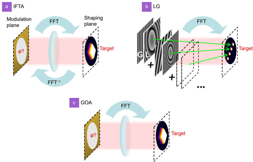
Fig. 3 | Main calculation strategies for determination of the spatial phase modulation \phi_M . (a) The iterative fourier transform algorithm (IFTA) based on FFT iterations between the modulation and the shaping planes. (b) The lens and grating (LG) calculation relies on the complex sum of phase masks to generate arrays of laser spots in 3D. (c) The global optimization algorithms encompasses all the strategies that permit to 'guess' the optimal \phi_M through stochastic optimization (simulated annealing, evolutionary algorithm etc.) or machine learning strategies (neural network etc.).
