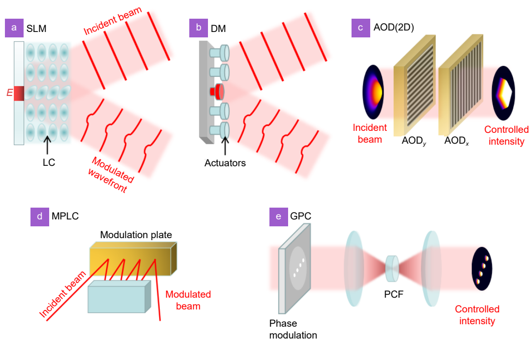
Fig. 2 | Main experimental systems for dynamic wavefront modulation. (a) Spatial light modulators (SLM) are based on a liquid crystal (LC) layer whose molecules can be orientated under an electric field E , permitting to dynamically control the spatial optical retardation of an impinging laser beam. (b) Deformable mirrors (DM) rely on a similar principle with actuators whose controllable height defines the optical retardation on the beam wavefront. They can be membrane-based or segmented. (c) The acousto-optic deflectors (AOD) are based on the generation of sound waves inside a crystal (e.g. \text{TeO}_2 or \text{PbMoO}_4 ). The related periodical variation of refractive index also permits wavefront modulation. (d) The multi-plane light conversion (MPLC) set-up is based on spatial mode conversion through successive passages on specifically designed phase retardation maps. (e) The general phase contrast method (GPC) relies on the principle of phase contrast microscopy where the transparent pure-phase sample corresponds to a controlled phase modulation (applied with an SLM for example) and the phase contrast filter (PCF) is the optical element turning this modulation into an intensity contrast in an imaging plane. See text for more details.
