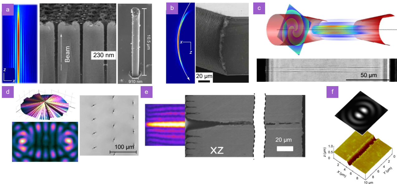
Fig. 6 | Surface and bulk structuring towards the sub micrometric scale using non-diffractive beams with the help of spatial beam shaping. (a) Bessel beam generation and high aspect ratio structuring of glass with single femtosecond pulses. (b) Turning non diffractive beam (or Airy beam) enabling curved machining of silicon. (c) Hollow core non-diffractive beam based on vortex phase modulation yielding tubular bulk photo inscription in a single irradiation. (d) Modulated axiconic phase mask forming a multiple lobes non diffractive beam permitting dynamic crack orientation control for glass cutting. (e) Drilling of stainless steel using non-diffractive beam with enhanced efficacy. (f) Machining of grooves using superimposed bessel beams associating an axicon and an SLM. Figure reproduced with permission from: (a) ref. 137 , the author, ref. 138 , under a Creative Commons Attribution License; (b) ref. 139 , the author; (c) ref. 140 , under a Creative Commons Attribution License; (d) ref. 141 , SPIE; (e) ref. 142 , under a Creative Commons Attribution License; (f) ref. 143 , the author.
