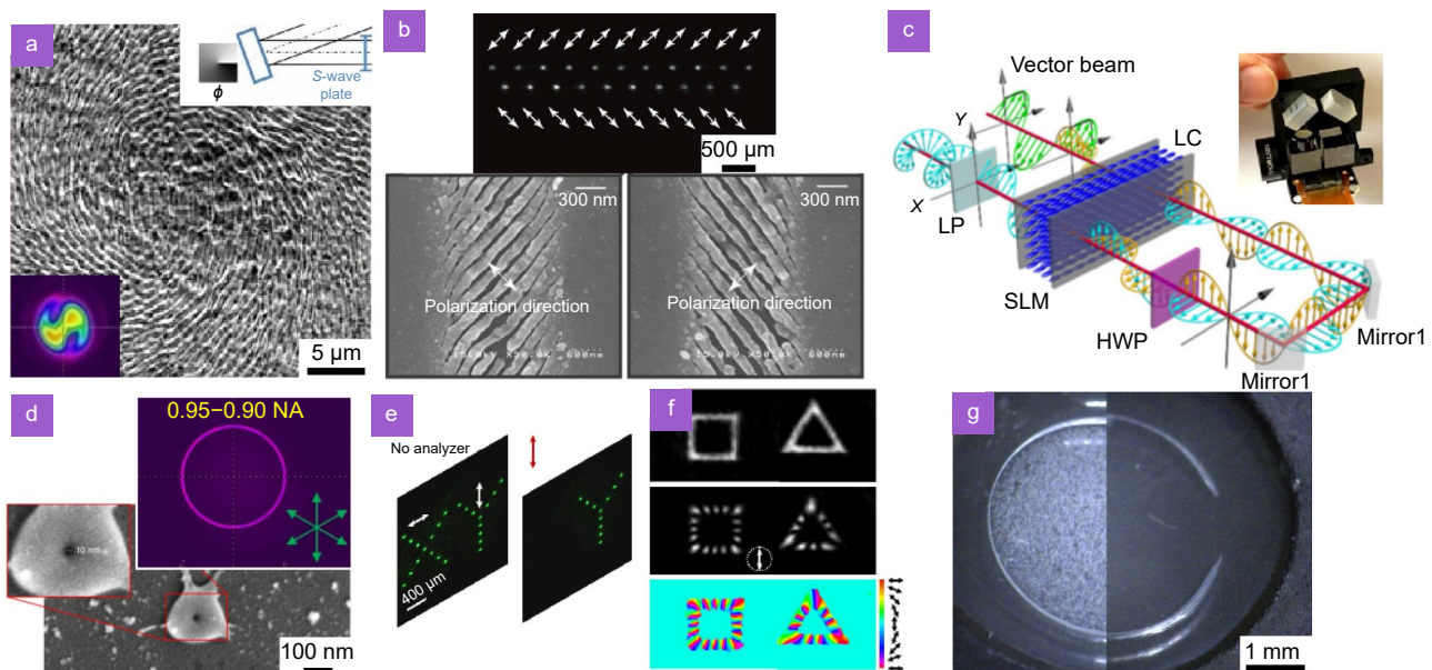
Fig. 7 | Spatial beam shaping with polarization control to achieve nanometric structuring. (a) Helical wavefront shaping using an SLM associated with an S-waveplate yielding a vortex beam generating spiral orientation of LIPSS on metal. (b) Array of laser spots with individual polarization control. The laser-induced surface tracks show the corresponding LIPSS orientation. (c) Example of integrated advanced dynamic polarization control using a single SLM. (d) 10 nanometer surface hole on sapphire combining annular beam shaping, polarization control and high numerical aperture focusing. (e) Generation of spot arrays in 3D with controlled polarization (not ultrafast laser). (f) Arbitrary intensity distribution controlled polarization distribution (not ultrafast laser). (g) Cutting of cornea using vortex beam shaping (right) compared with regular Gaussian beam (left) showing a smoother and more precise cut. Figure reproduced with permission from: (a) ref. 157 , the author; (b) ref. 158 , the author; (c) ref. 159 , (d) ref. 160 , under a Creative Commons Attribution License; (e) ref. 161 , the author; (f) ref. 162 , the author; (g) ref. 163 , under a Creative Commons Attribution License.
