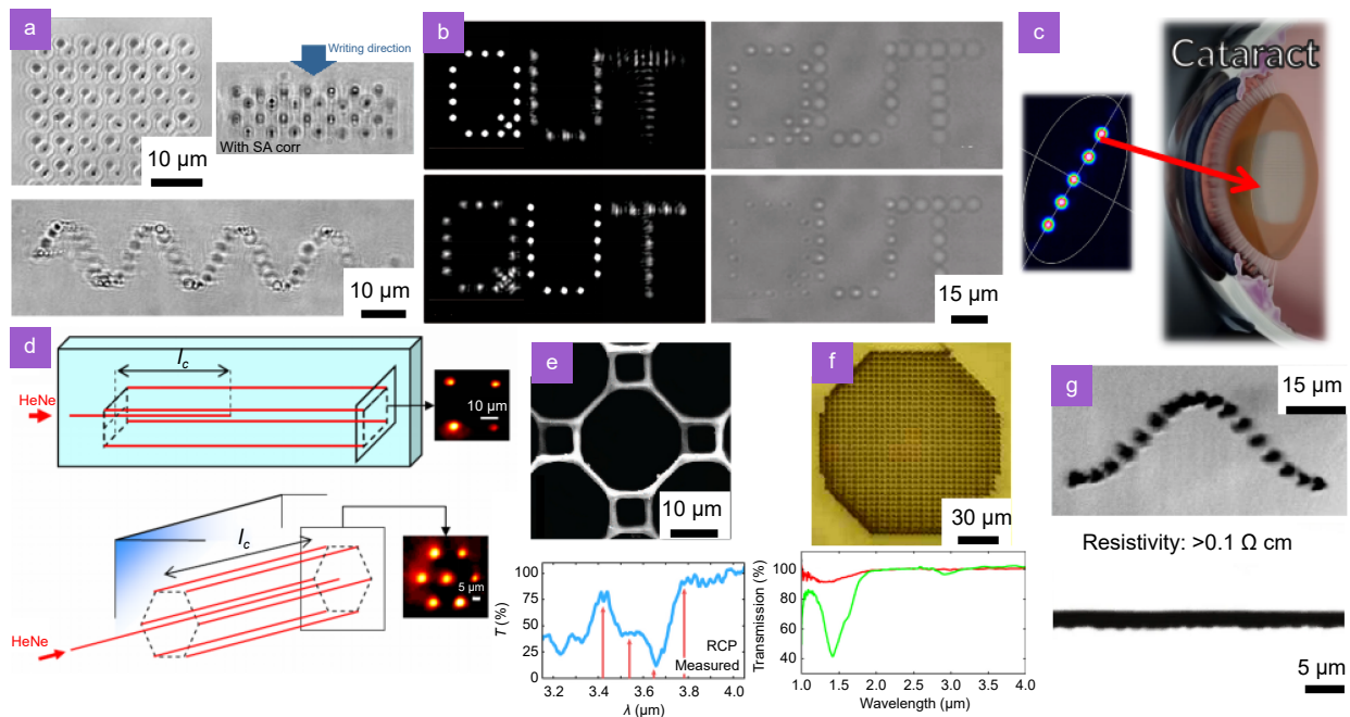
Fig. 5 | Examples of ultrafast laser bulk photoinscription with the help of spatial beam shaping. (a) Structuring of glass at the microscale level using 3D arrays of spots achieved in a single irradiation using LG algorithm including depth-related aberration correction. (b) Photoinscription in glass using the fractional Fourier transform iterative algorithm generating arrays of laser spots in multiple planes. (c) Photo emulsification of the crystalline lens for the cataract surgery with the help of spatial beam shaping of ultrafast laser. (d) Photoinscription of photonic devices inside fused silica with optical functions (here light division). (e) Fabrication of gyroid photonic crystals using wavefront compensation of the depth-related strong spherical aberration in chalcogenide glass generating circular dichroism (RCP: right handed circular polarization). (f) Photonic crystal in lithium niobate with adaptive control of the wavefront to compensate for the spherical aberrations. (g) Structuring of diamond in three dimension yielding conductive wires in the bulk. Figure reproduced with permission from: (a) ref. 95 , the author; (b) ref. 122 , the author; (c) ref. 9 , the author, ref. 123 , under a Creative Commons Attribution License; (d) ref. 124 , Optical Society of America; (e) ref. 125 , the author; (f) ref. 126 , the author; (g) ref. 95,127 , the author.
