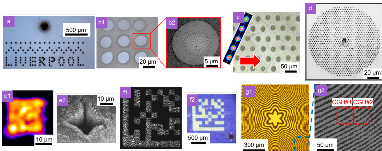
Fig. 4 | Surface structuring with dynamic wavefront shaping. (a) Array of impacts on silicon using 15 irradiation steps, the unwanted 0 th order leaves a strong crater at the top of the array. (b1) Parallel structuring of tempered glass using an array of 6 laser spots with anti-reflection properties due to the LIPSS (b2). (c) Combination of multispot shaping and beam scanning for stainless steel surface processing conferring friction reduction properties. (d) Reaching more than 1000 laser spots in a single irradiation on glass (Schott B270), note the effect of the unwanted 0 th order. (e1) Square top hat beam with corresponding crater on steel (e2). (f1) Shaping of arbitrary intensity distributions with the detrimental speckle effect and its marking on photoresist (f2) with a strong crater at the 0 th order position (bottom right). (g1) Fresnel zone plate fabrication by successive shaped beam irradiations (g2) stitched together on Au film on SiO 2 . Figure reproduced with permission from: (a) ref. 37 , the author; (b) ref. 102 , (c) ref. 103 , under a Creative Commons Attribution License; (d) ref. 48 , Optical Society of America; (e) ref. 35 , the author; (f) ref. 104 , the authors; (g) ref. 105 , under a Creative Commons Attribution License.
