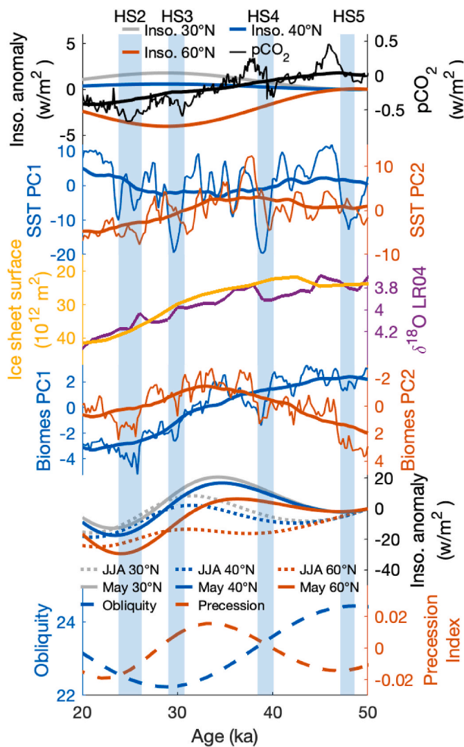
Fig. 4. Mean annual insolation anomaly as compared to 50ka configuration at 30°N, 40°N and 60°N (Berger, 1978; Berger and Loutre, 1991; Huybers and Eisenman, 2006), pCO 2 forcing anomaly as compared to 50ka (thick black line shows the 10ka window running mean (Bereiter et al., 2015)); sea surface temperature PC1 and PC2 (thick lines show the 10ka window running mean of the PC1 and PC2). Eurasian ice sheet surface (Gowan et al., 2021) and LR04 benthic δ 18 O stack (Lisiecki and Raymo, 2005); Tf/nTf PC1 and PC2. Mean insolation anomaly for summer (JJA) and May at 30°N, 40°N and 60°N; and obliquity and precession index.
