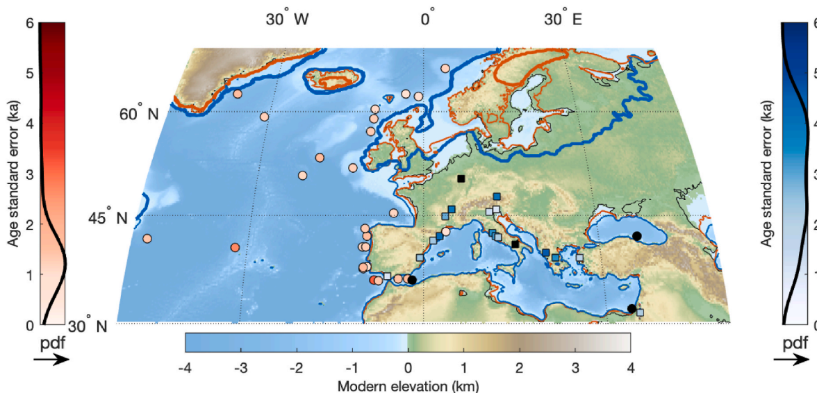
Fig. 1. Mean standard error of age model for continental (square, blue scale) and marine (dots, red scale) archives for the 50–20 ka period. Probability density function of mean standard error for marine and terrestrial archives are also displayed in their respective color bar. Black filling indicates archives for which the age model was reproduced from the original publication. Red and blue thick lines show ice sheet extension at 50 ka and LGM respectively (Gowan et al., 2021). The thin red and blue lines represent coastlines at 50 and 20 ka respectively (Gowan et al., 2021).
