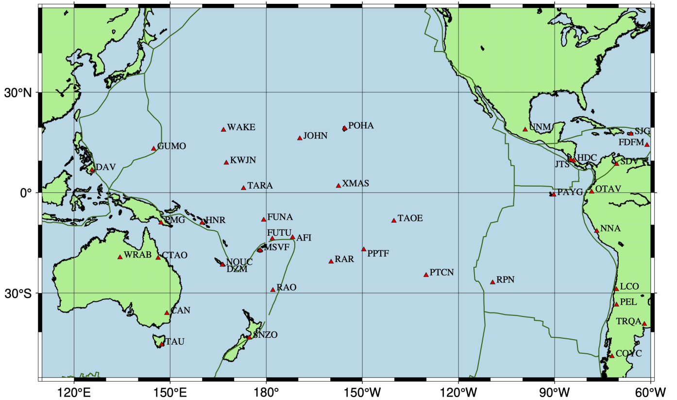
Figure 3 Locations of the 40 surface (land) stations used to compare waveforms.
