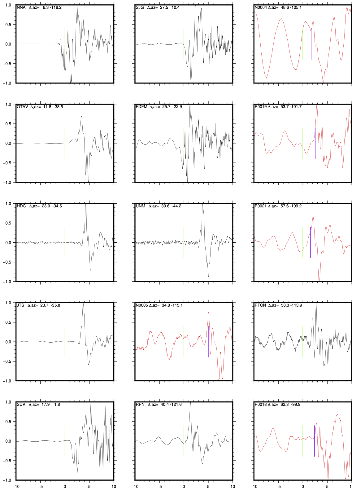
Figure 5 Seismograms for the event of 2022/06/08 plotted in an order that allows for easy comparison of waveforms at nearby stations. Epicentral distance \Delta and azimuth are plotted in the upper left corner. The green line indicates the expected P wave arrival (using model AK135), purple lines those of the AIC pick from Simon et al. (2020) in MERMAID seismograms. To distinguish them from surface stations, MERMAID seismograms are coloured red.
