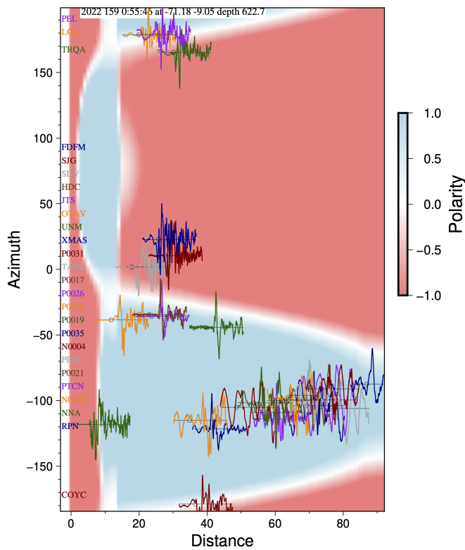
Figure 6 Predicted polarity (UP=blue) for event 2022/06/08 ( 71^{\circ}\text{W} , 9^{\circ}\text{S} , 622 km depth). Small circles indicate distance and azimuth, plotted at the expected arrival time of the P wave. Many overlapping seismograms are hard to distinguish even when plotted in different colours, but are nevertheless shown, simply to indicate the coverage of MERMAIDs and island records in the distance/azimuth plane.
