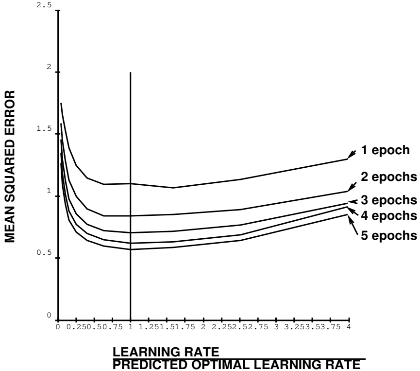
Fig. 1.25. Mean squared error as a function of the ratio between learning rate and predicted optimal learning rate for a fully connected network ( 784 \times 30 \times 10 ). The training set consists of 300 handwritten digits.
