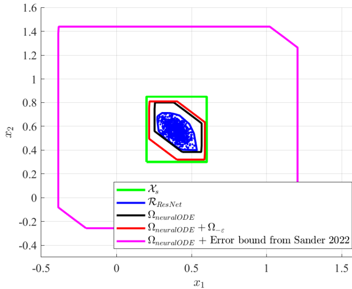
Fig. 5. Verification of ResNet based on neural ODE
