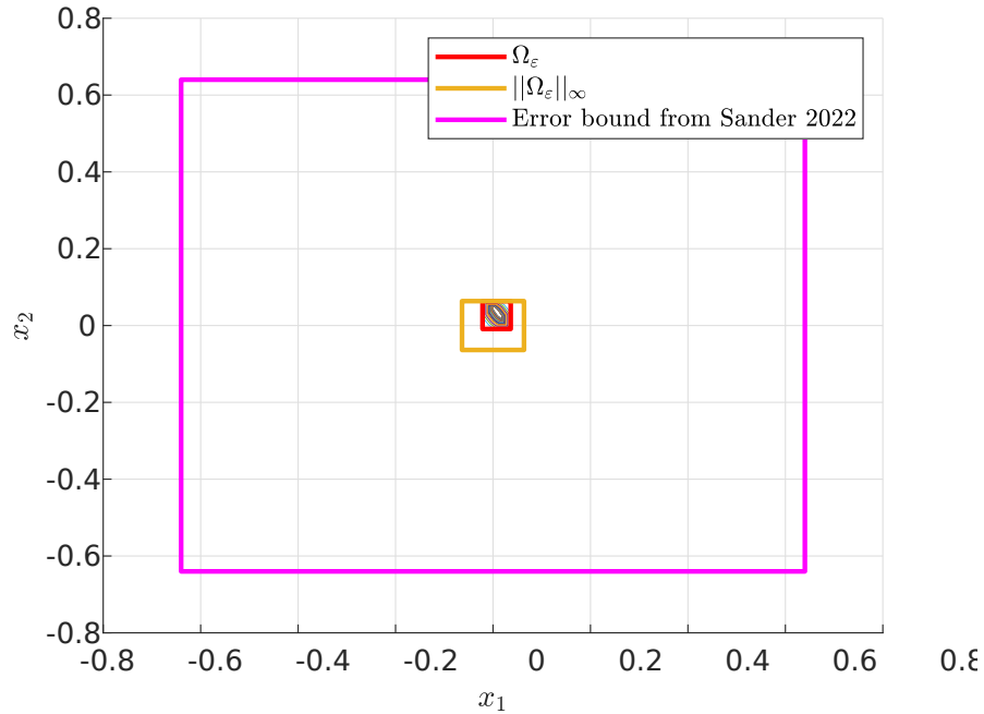
Fig. 3. Comparison of the error bounds obtained from our approach in red and the one from [26] in magenta
