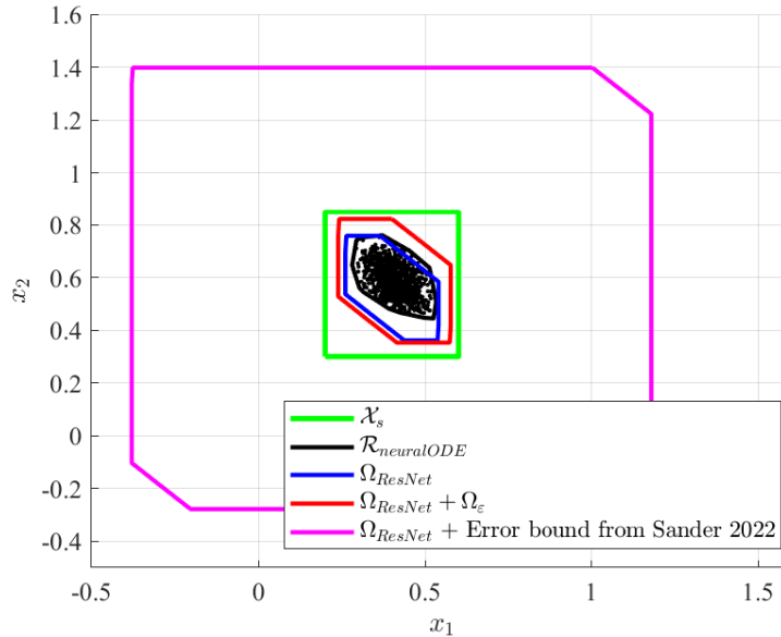
Fig. 4. Verification of neural ODE based on ResNet
