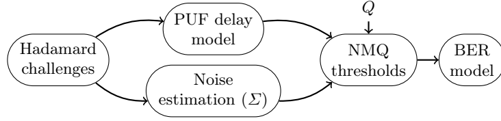
Fig. 7: BER estimation for Neyman-Pearson PUF Authentication Protocol
