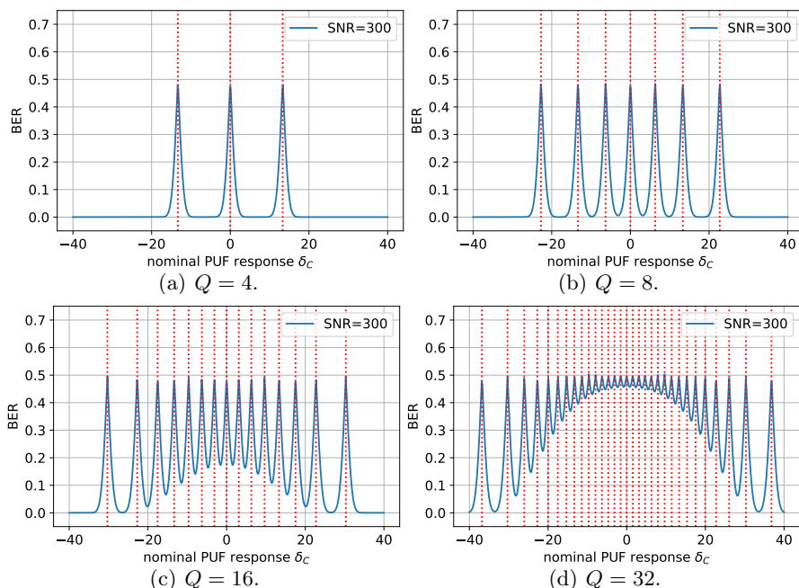
Fig. 2: BER estimation for different quantization levels and \text{SNR} = 300 .
