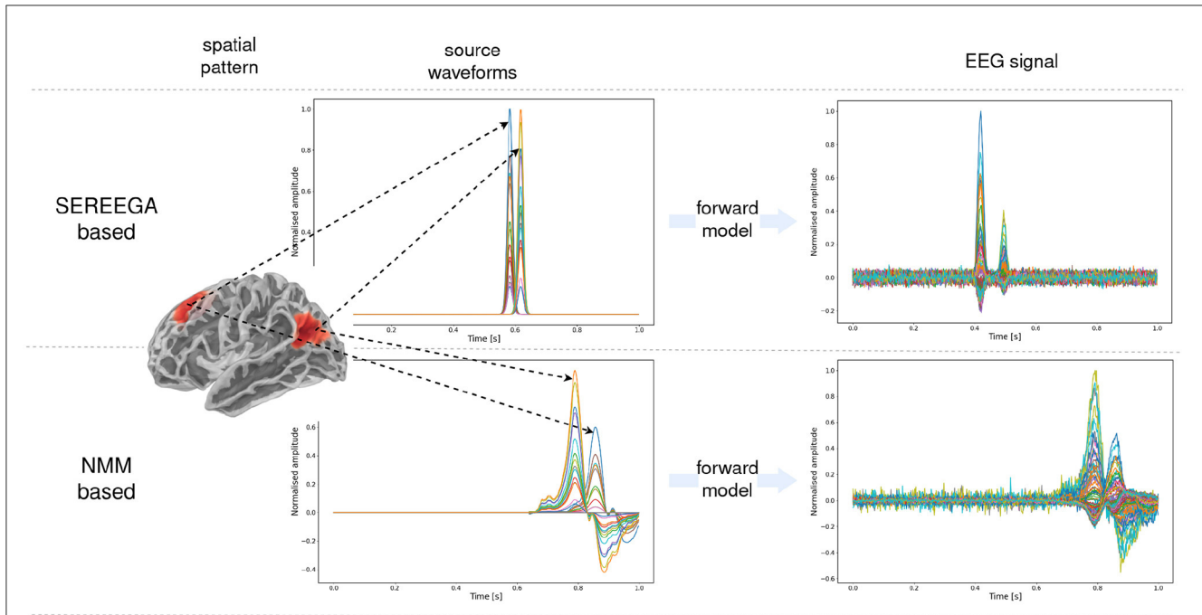
FIGURE 2 Simulated data with the two different types of simulation: SEREEGA based and NMM based. Visualization of the waveform of active sources and the final EEG data obtained through the forward model. For the NMM based simulation, the simulated source activity contains signals for active sources (spikes) and noise sources. The generated EEG corresponds to the projection of this “noisy” source activity. However the ground truth source data that is used for training corresponds to a “denoised” source activity where all non-active regions are set to zero.
