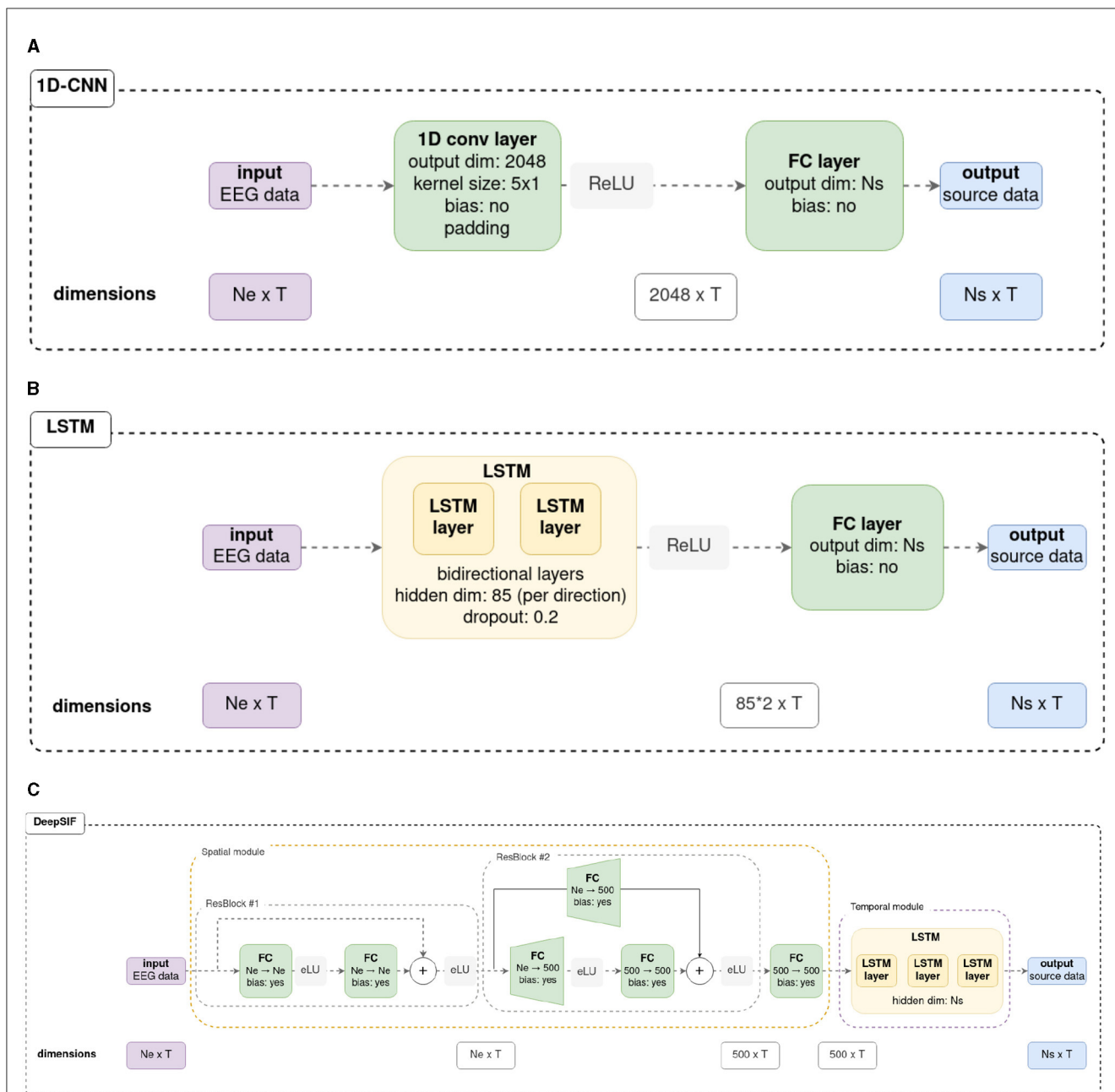
FIGURE 1 Details of the three neural networks used in this work. Original schemes for the LSTM and deepSIF architectures can be found in these original articles (Hecker et al., 2022; Sun et al., 2022). For the neural networks in Sections 3.1, 3.2, N_e = 90 , N_s = 994 and T = 500 . For the neural networks trained in Section 3.3, N_e = 59 , N_s = 1,176 , and T = 500 . (A) 1D-CNN architecture details. (B) LSTM from Hecker et al. (2022) architecture details. (C) deepSIF, spatio-temporal network from Sun et al. (2022) architecture details.
