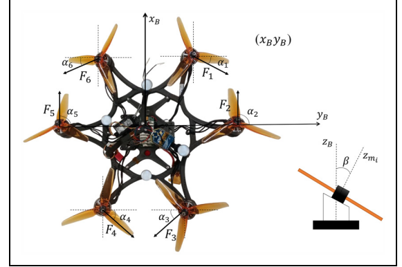
Figure 2. Forces projection in the lateral plane with the motor tilting angles \beta between z_B and z_{m_i} the axis of the i -th motor.
