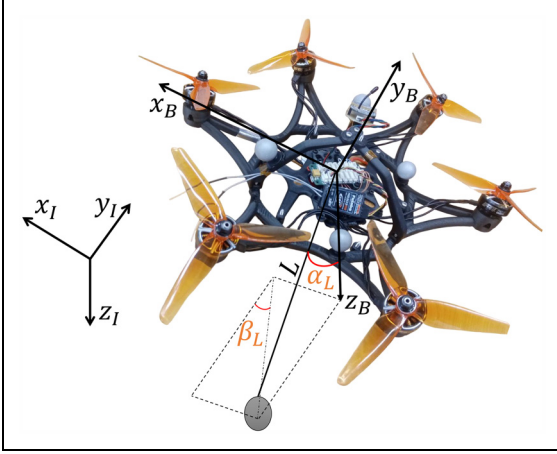
Figure 1. Fully Actuated Hexacopter attached to a payload with Inertial ( \mathcal{F}_I ) and Body ( \mathcal{F}_B ) Frames. The cable suspended pendulum is described by two angles \alpha_L and \beta_L along the z -axes and the inertial lateral plane ( x_I y_I ) respectively.
