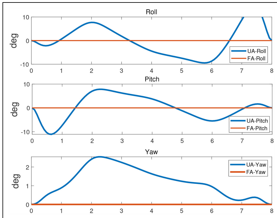
Figure 4. Euler angles comparison between FA-Hex and UA-Hex.
