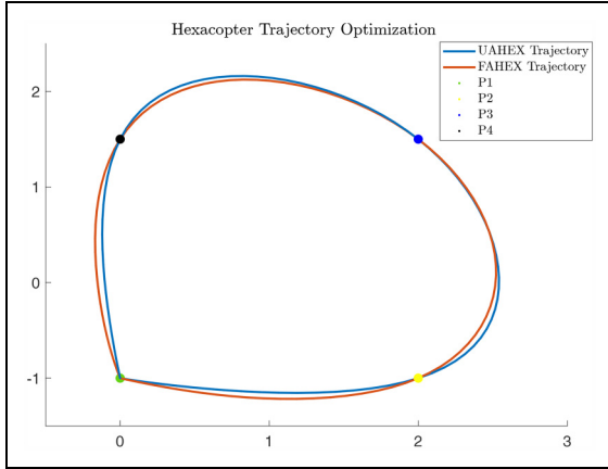
Figure 3. Projection in the horizontal plane of the optimized trajectory for FA-Hex and UA-Hex drones as they fly between specified points and then return to their initial positions. The points are defined by their coordinates: P1 = [0, -1, 1.3] , P2 = [2, -1, 1.3] , P3 = [2, 1.5, 1.8] and P4 = [0, 1.5, 1.8] .
