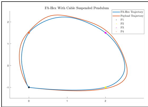
Figure 5. Projection in the horizontal plane of the optimized trajectory for FA-Hex with cable suspended pendulum.
