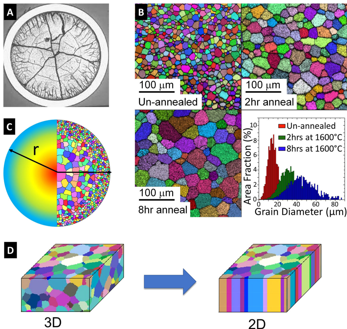
Fig. 1 | Variation of \text{UO}_2 grain size within nuclear fuel and replication method.
