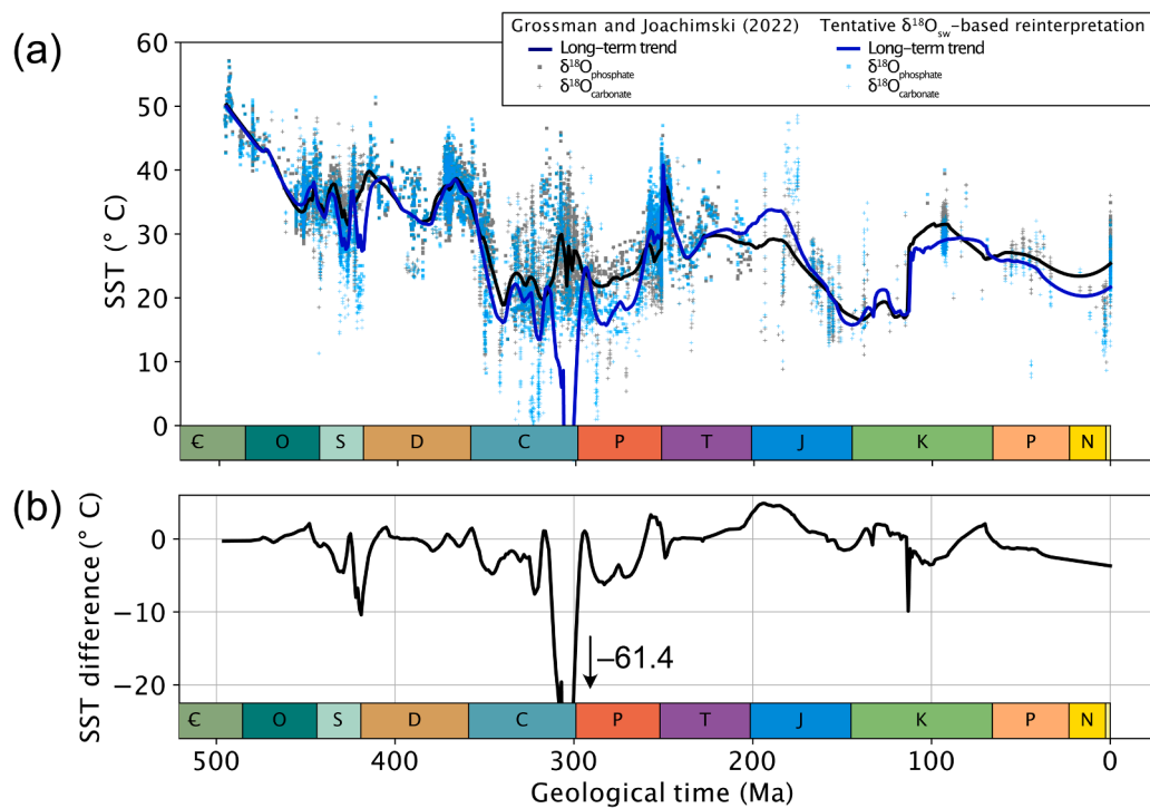
Fig. 8. Model-informed Phanerozoic SST reconstruction. (a) Low-latitude ( \sim 30^{\circ}\text{N} ) SST reconstruction derived from the quality-controlled \delta^{18}\text{O}_{\text{carbonate}} (cross markers) and \delta^{18}\text{O}_{\text{phosphate}} (square markers) data of the StabisoDB database as per the original calculations of Grossman and Joachimski (2022) (black markers and line) vs. using for each data point the \delta^{18}\text{O}_{\text{sw}} value averaged over the closest oceanic grid point and immediately adjacent grid points in the closest of the 109 Phanerozoic HadCM3 time slices considered (blue markers and line). (b) Difference induced by using the \delta^{18}\text{O}_{\text{sw}} value averaged over the closest oceanic grid point and immediately adjacent grid points in the closest of the 109 Phanerozoic time slices considered, instead of the original calculations of Grossman and Joachimski (2022) (i.e., blue minus black lines of panel (a)). Calculations were conducted using the HadCM3 climatic simulations, the \delta^{18}\text{O}_{\text{sw}} -salinity relationship of Railsback et al. (1989), the temperature- \delta^{18}\text{O}_{\text{phosphate}} relationship of Puc at et al. (2010) and the temperature- \delta^{18}\text{O}_{\text{carbonate}} relationship of Kim and O’Neil (1997). C: Cambrian; O: Ordovician; S: Silurian; D: Devonian; C: Carboniferous; P: Permian; T: Triassic; J: Jurassic; K: Cretaceous; P: Paleogene; N: Neogene.
