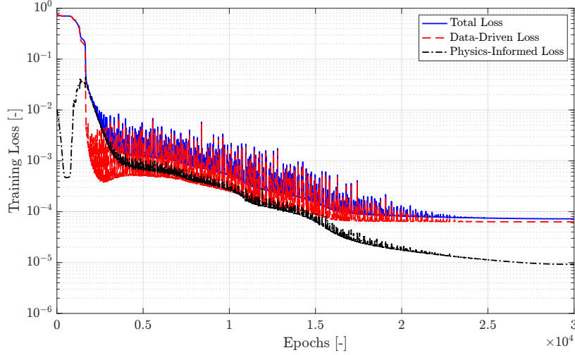
Figure 15: Evolution of the different loss functions when training is performed considering experimental data. Here, the neural networks of \hat{E}_r and \hat{\eta} are composed by a single biases.
