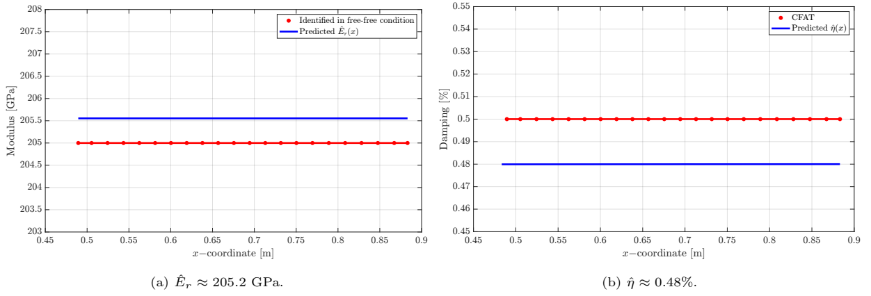
Figure 17: Predictions of \hat{E}_r and \hat{\eta} parameters when considering the experimental data around the 11th bending mode. — represents the neural network’s predictions, whereas • represents the behavior of the material properties across the beam identified by benchmark methods.
