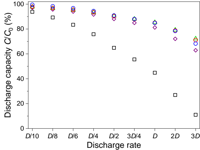
Figure 7. Power signature curves at 25 °C- Discharge capacities of C2400 (open black squares) and functionalized separators C6 (open purple diamonds), C7 (open green triangles), C8 (open red hexagons) and C9 (open blue circles) as a function of the discharge rate.
