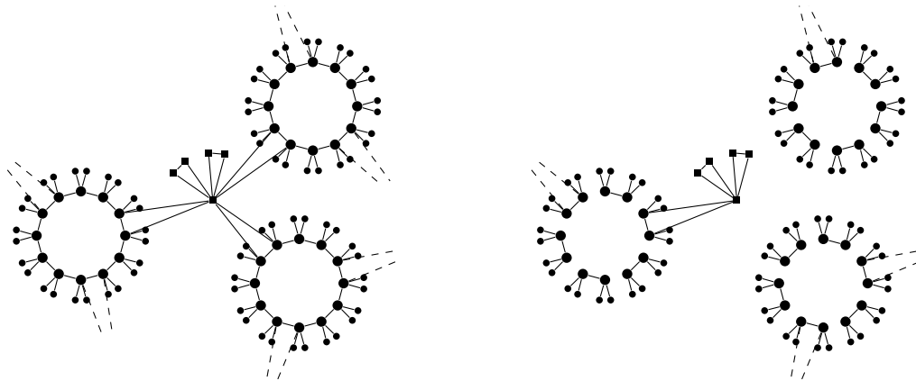
(a) A part of the graph G : the clause gadget is connected to three variable gadgets. The dashed edges indicate that they may be connected to other clauses. (b) A possible correction of the graph G . Only one variable gadget remains connected to the clause gadget. One edge out of two of the cycle of a variable gadget is deleted.
