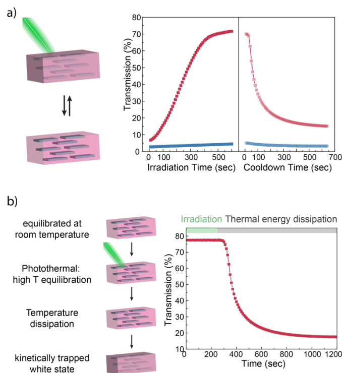
Figure 4. Photo-thermally induced phase transition of AuNPs containing ZB-hectorite hydrogels. a) Upon irradiation a hydrogel preconditioned at 50 °C undergoes turbid-transparent transition through photo-thermal heat build-up. In the absence of light irradiation (red), the hydrogel returns quickly back to its opaque state. In absence of AuNPs no phase transition occurred (blue). b) A room temperature equilibrated, and transparent hydrogel undergoes no visible optical change upon irradiation. After short time of removal of light source, the hydrogel turns opaque due to thermal conditioning.
