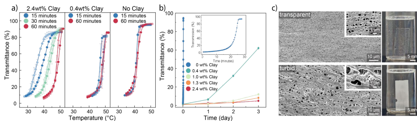
Figure 3. Influence of large aspect ratio hectorite clay on equilibration kinetics. a) The presence of hectorite clay leads to significantly slower equilibration kinetics during upward equilibration to 50 °C. In absence of clay, equilibration is fast but transition temperature is around 10 °C lower than heating temperature. The data are mean values with standard deviations as error bars from 3 measurements. b) In absence of clay, the downward equilibration kinetics is fast, whereas small amounts of clay lead to much slower kinetics in the range of days. c) Scanning electron micrographs and optical photographs of transparent and turbid hydrogels reveal the size difference of polymer- and water-rich domains leading to strong scattering in the case of the turbid gel.
