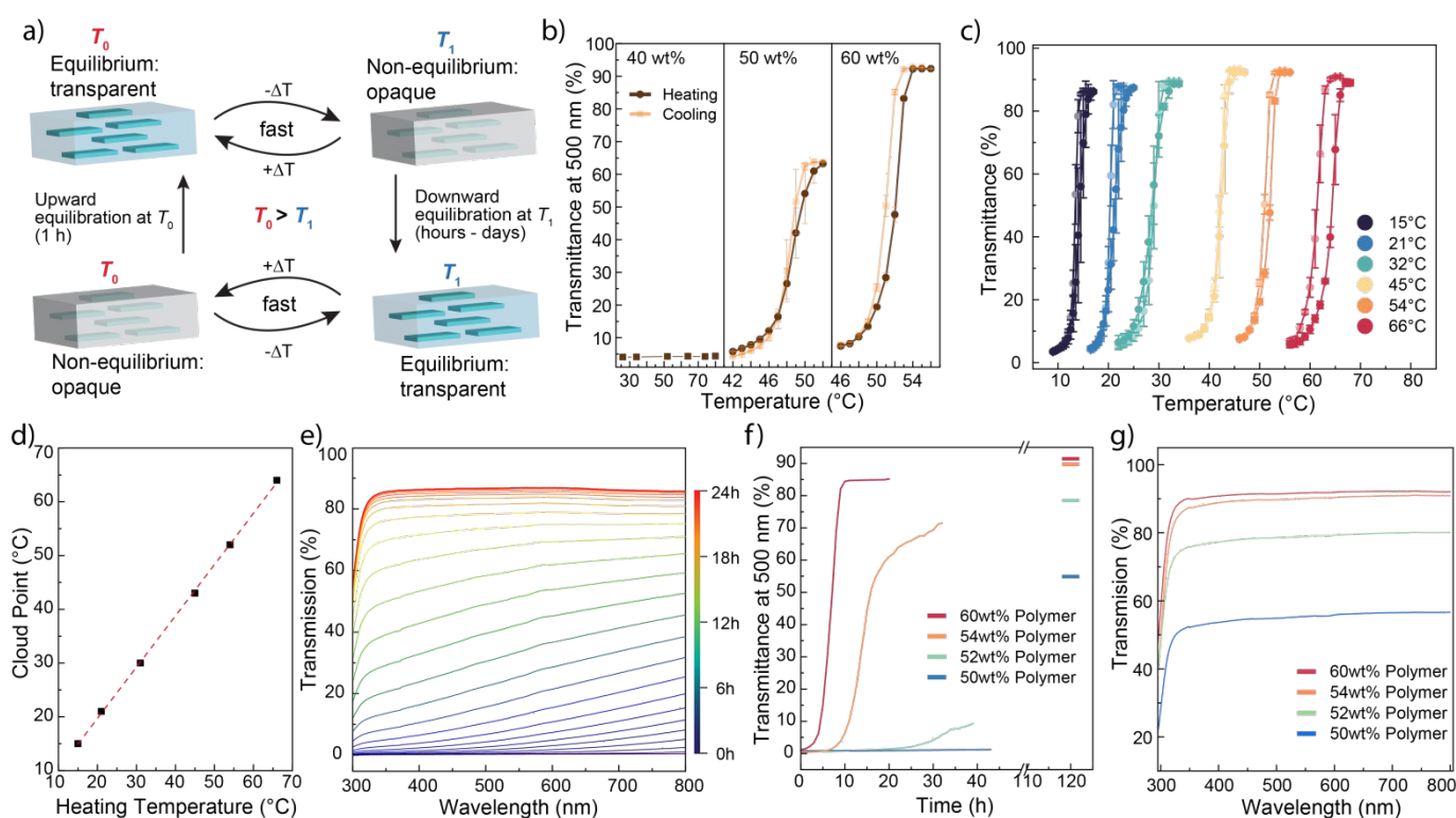
Figure 2. Characterization of phase transitions of hydrogels. a) Overview of fast phase transition response between non-equilibrium and equilibrium state. Downward equilibration indicates equilibration from a higher temperature T_0 to a lower temperature T_1 , while upward equilibration indicates equilibration from a lower temperature to a higher temperature. Fast change of temperature around equilibration temperature allows swift response without affecting the UCST. b) Optical response of hydrogels equilibrated at 53 °C for different polymer wt%. The data are mean values with standard deviations as error bars from 3 measurements. c) Upon equilibration for 1h at the indicated temperatures, the cloud point of the hydrogel adjusts itself to just slightly below the equilibration temperature. Polymer content: 60 wt%. The data are mean values with standard deviations as error bars from 3 measurements. d) The resulting cloud points correlate well with the equilibration temperature. e) Exemplary kinetic course of downward RT equilibration of a 60 wt% hydrogel after 15 min at 60 °C. f) The recovery after 15 min 60 °C depends on the polymer wt% of the hydrogel. g) Hydrogels with higher Polymer wt% show higher optical transparency.
