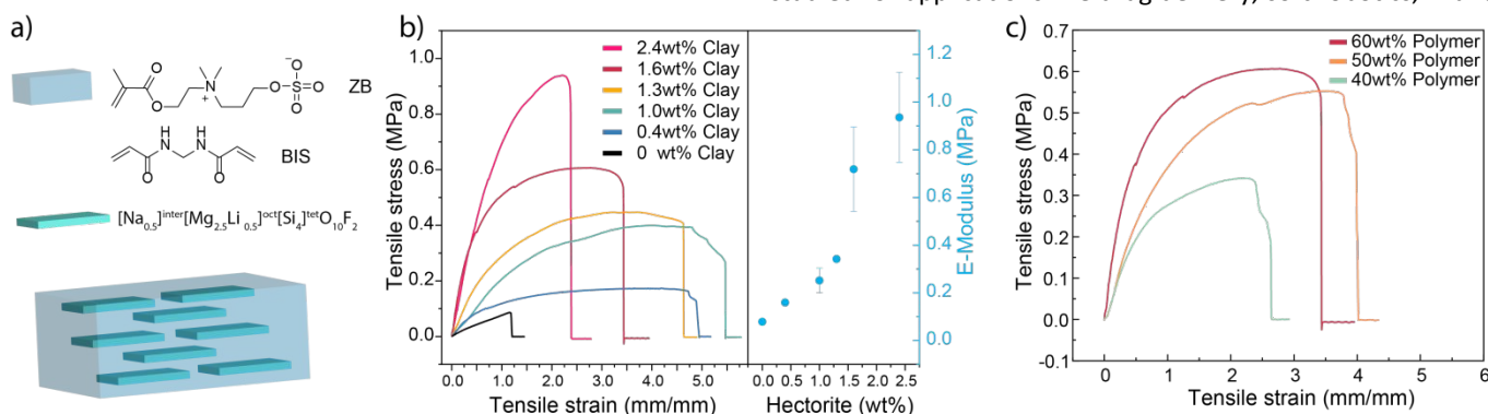
Figure 1. Zwitterionic hydrogels containing high aspect ratio hectorite clays. a) Chemical structures of the ZB monomer, chemical crosslinker and hectorite nanosheet. b) Mechanical properties of hydrogels with 60 wt% ZB content, 0.1 g/L BIS and various wt% of hectorite. c) Mechanical properties of various polymer wt% and 1.6 wt% clay.
