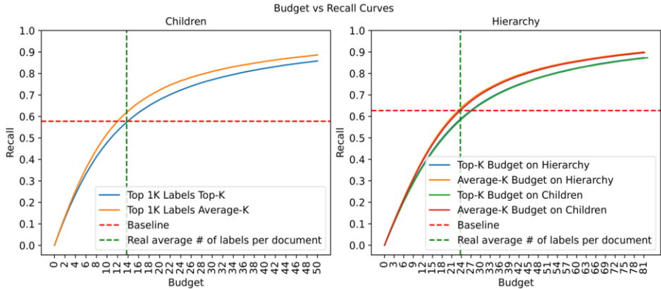
Figure 1. Top- K vs Average- K . In the left graph, we only consider leaf nodes. In the right graph, we consider the hierarchy.
