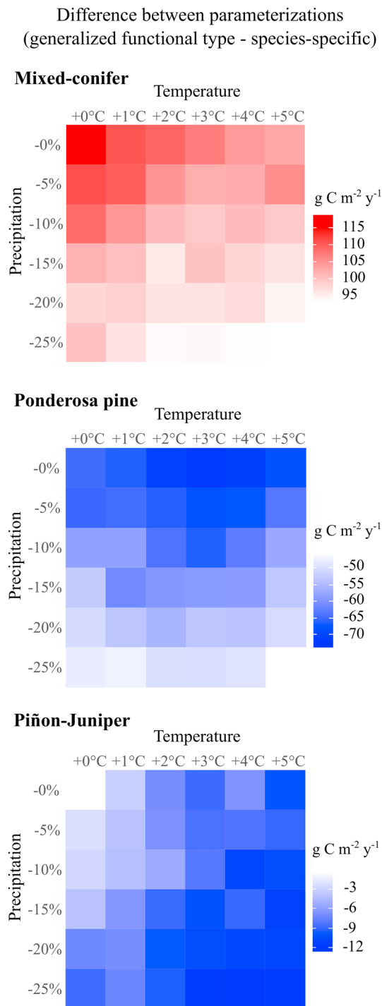
Figure 4. Difference between the annual net photosynthesis simulated with the generalized parameterization and with the species-specific parameterization at the three sites under different climate scenarios (see figure S2 for original simulated values from both parameterizations). Values correspond to the mean of the last decade of the 30 replicate 200-year simulations.
