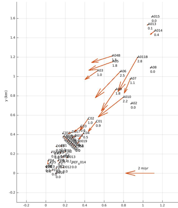
Figure 13. Horizontal velocities (m/year) for the period 2021 to March 2023 at the La Valette landslide (France). Grid is every 0.2 km
