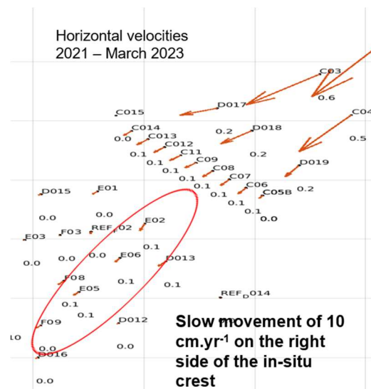
Figure 14. 2021-2023 velocity vectors and magnitude (m/yr) of the lower part of the La Valette landslide (France).
