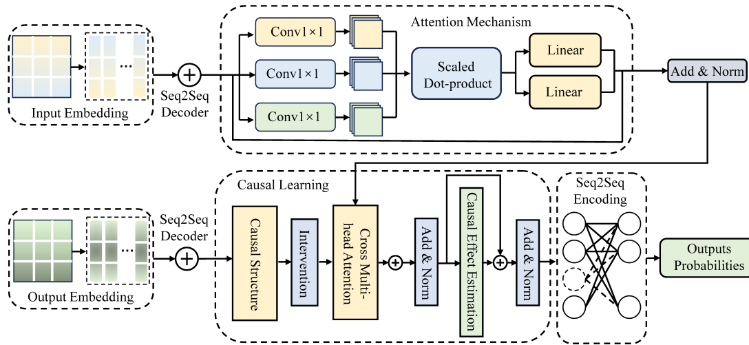
Figure 1. Overall algorithm architecture.
