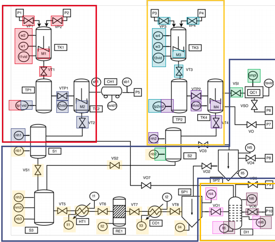
Figure 18: Division of the Tennessee Eastman Chemical Process by Sub-processes
