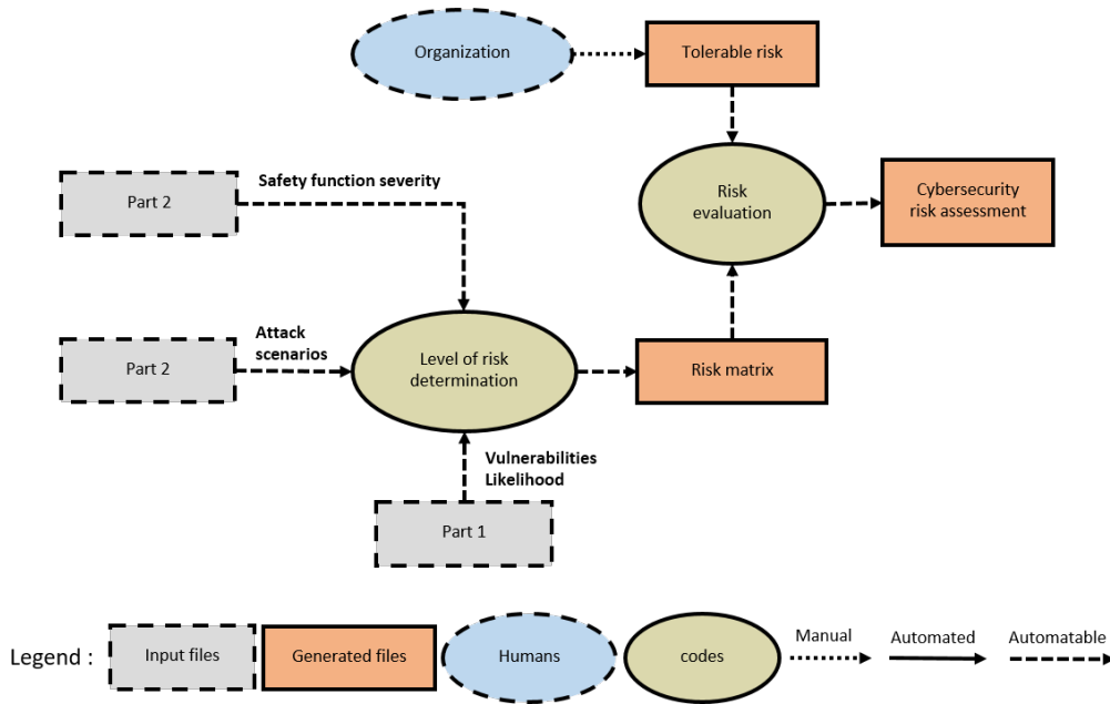
Figure 11: Part 3 process and automation
