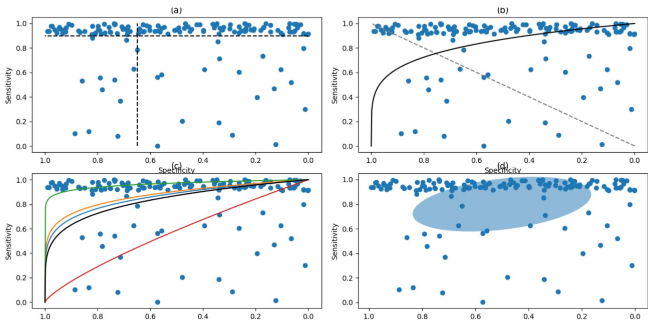
Fig. 4 Graphical display of d-dimer for deep vein thrombosis meta-analyses results. Source: Fig. 1 of Sutton et al. [56]
