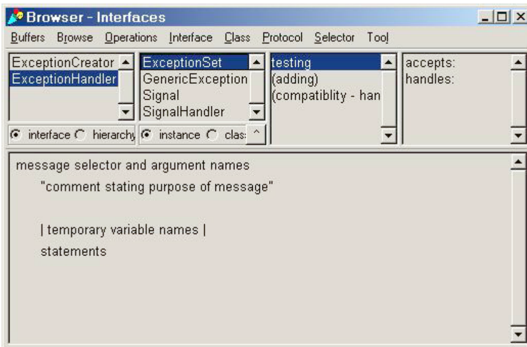
Figure 4: Interface views for classes implementing ExceptionHandler.
