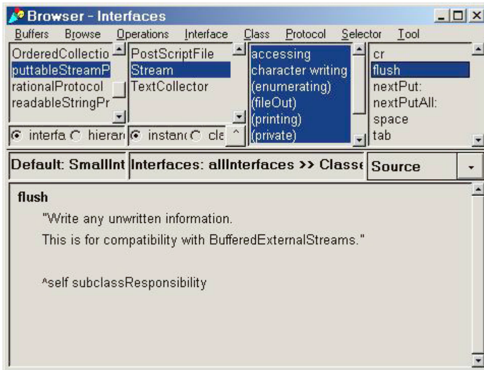
Figure 5: puttableStreamProtocol view of Stream.
