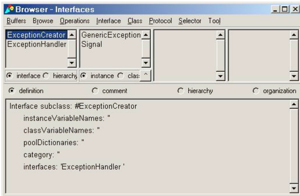
Figure 3: ExceptionCreator definition and classes implementing it.
