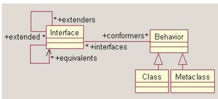
Figure 1: Relationships between Interfaces and Classes.
