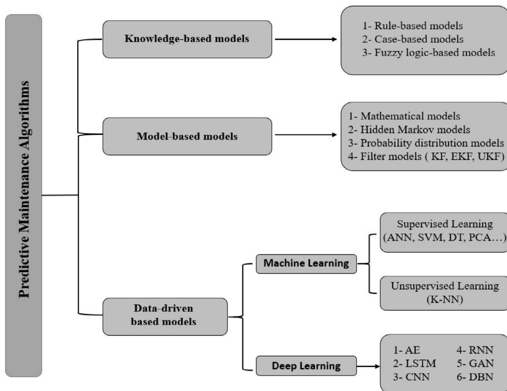
Fig. 1. Predictive maintenance algorithms.
